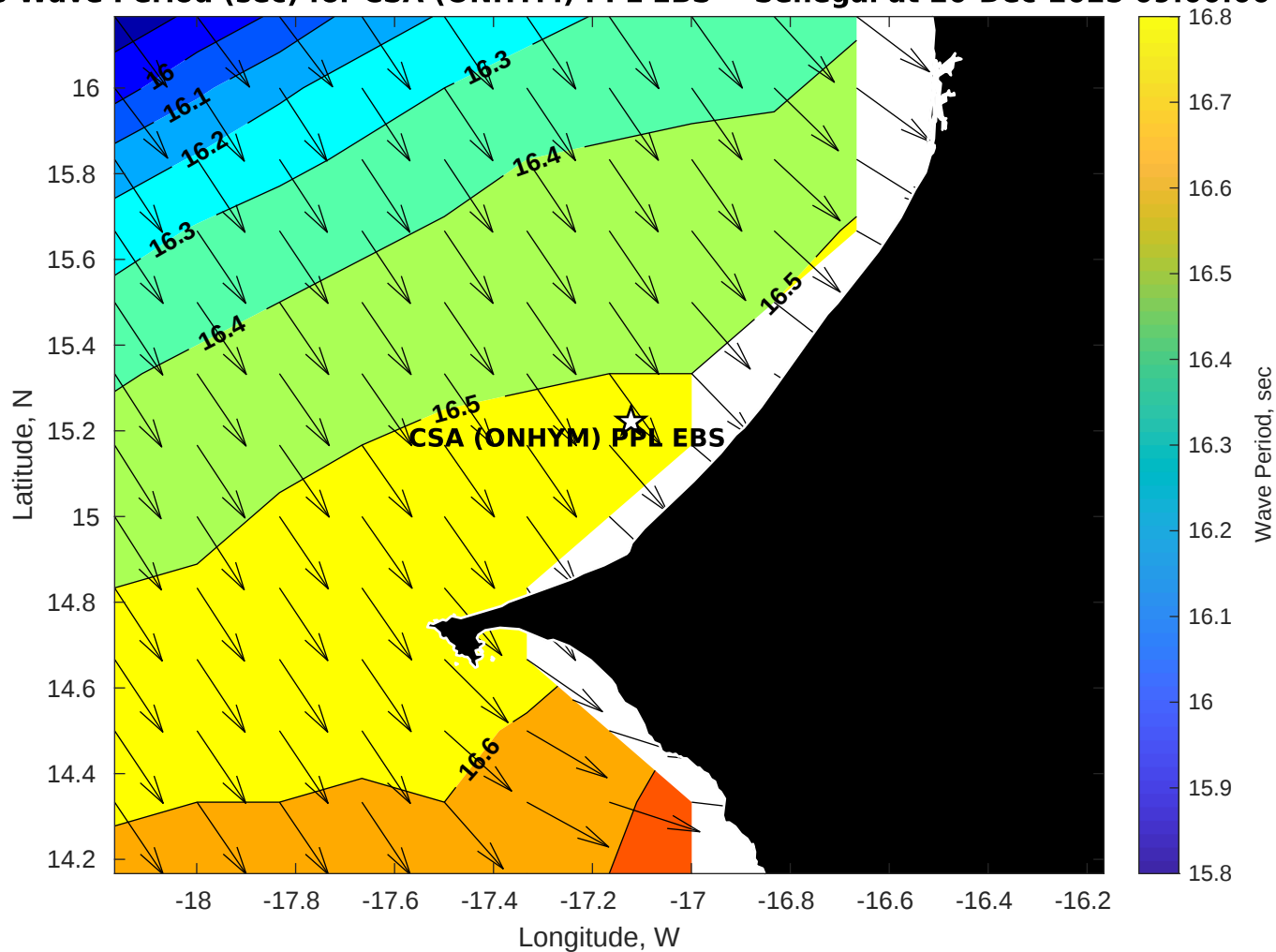
GFS Wave Period (sec) for CSA (ONHYM) PPL EBS - Senegal at 20-Dec-2025 09:00:00
