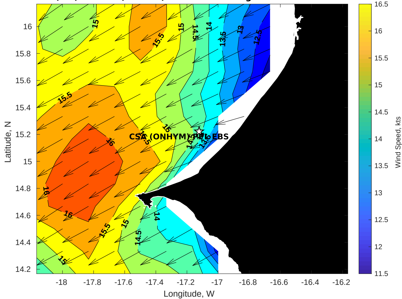
GFS Winds (kts) for CSA (ONHYM) PPL EBS - Senegal at 20-Dec-2025 09:00:00
