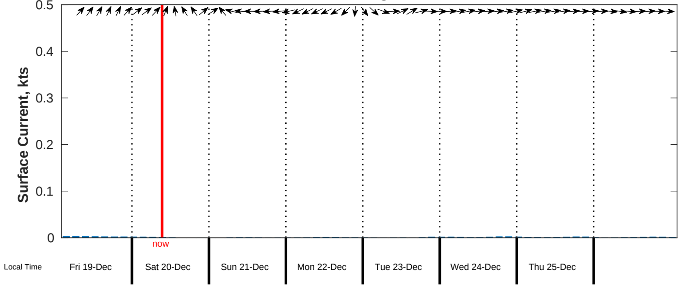
Surface Current Forecast for CSA (ONHYM) PPL EBS - Senegal from 19-Dec-2025 00:00:00 to 27-Dec-2025 00:00:00
