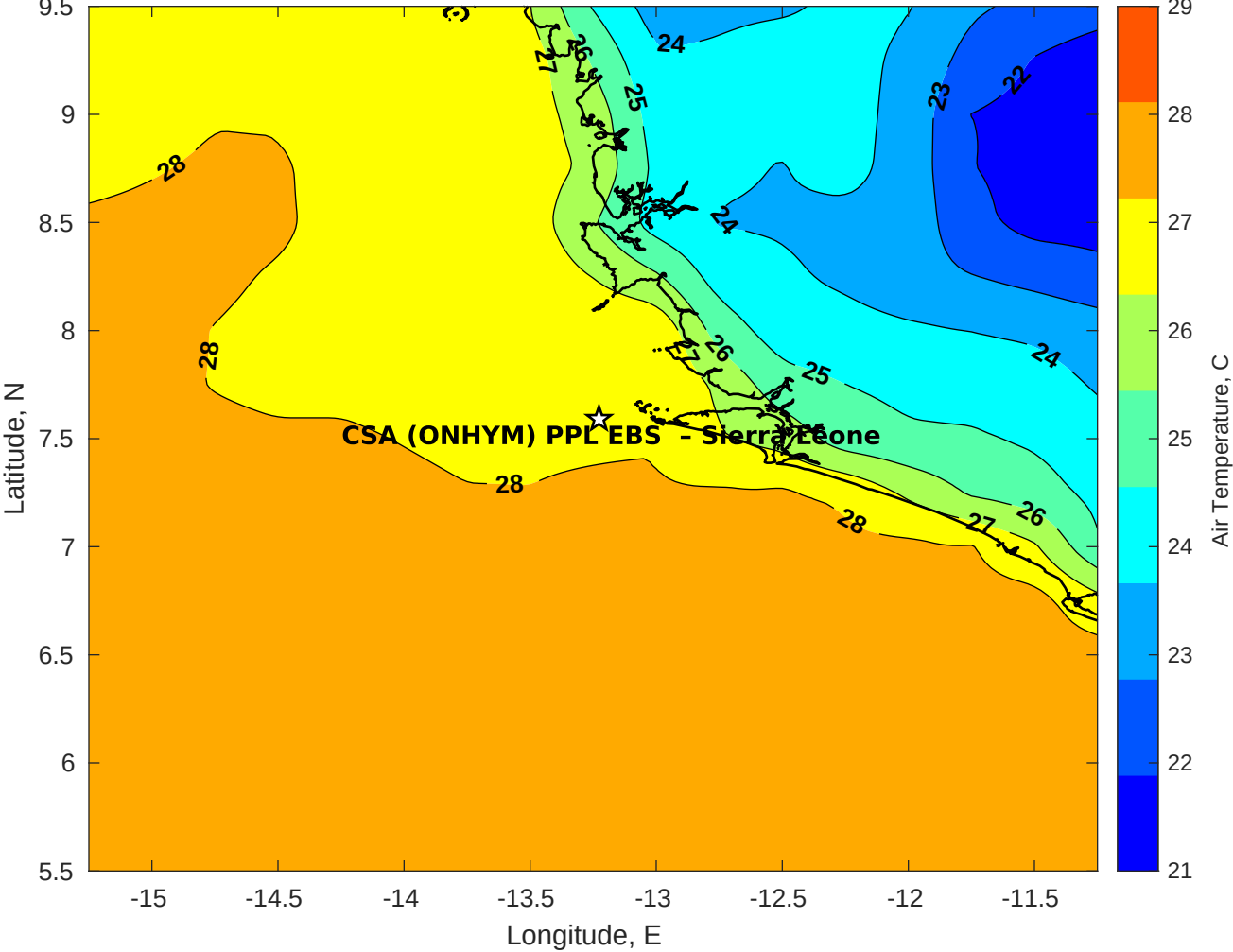
Air Temperature (C) for CSA (ONHYM) PPL EBS - Sierra Leone at 20-Dec-2025
