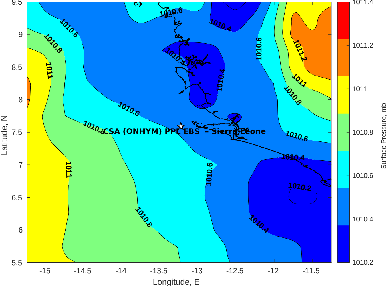
Surface Pressure (mb) for CSA (ONHYM) PPL EBS - Sierra Leone at 22-Dec-2025 00:00:00
