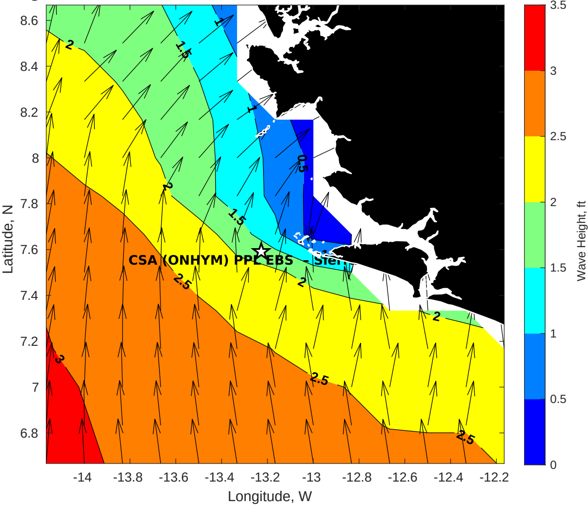
GFS Wave Height (ft) for CSA (ONHYM) PPL EBS - Sierra Leone at 20-Dec-2025 09:00:00
