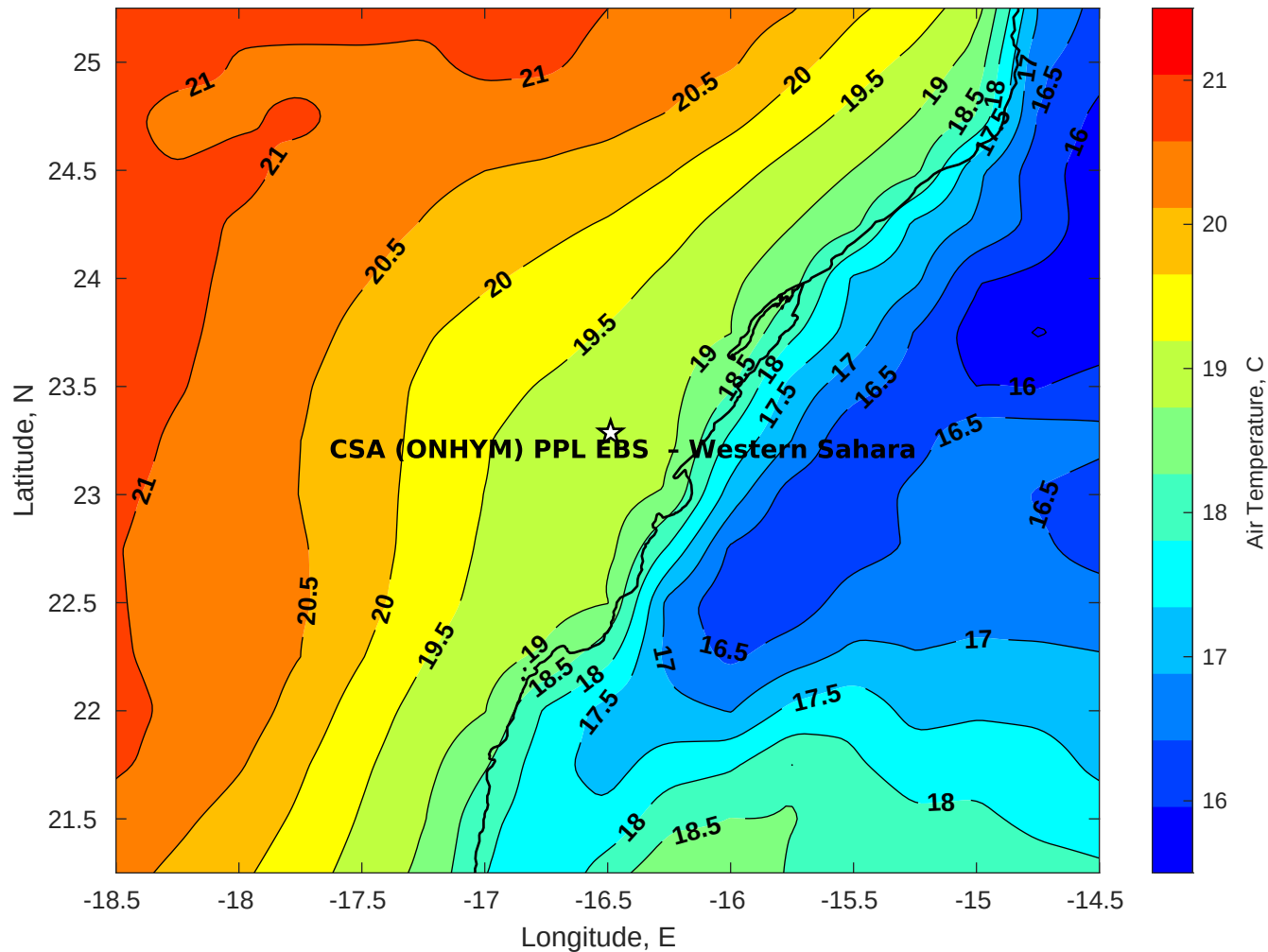
Air Temperature (C) for CSA (ONHYM) PPL EBS - Western Sahara at 20-Dec-2025
