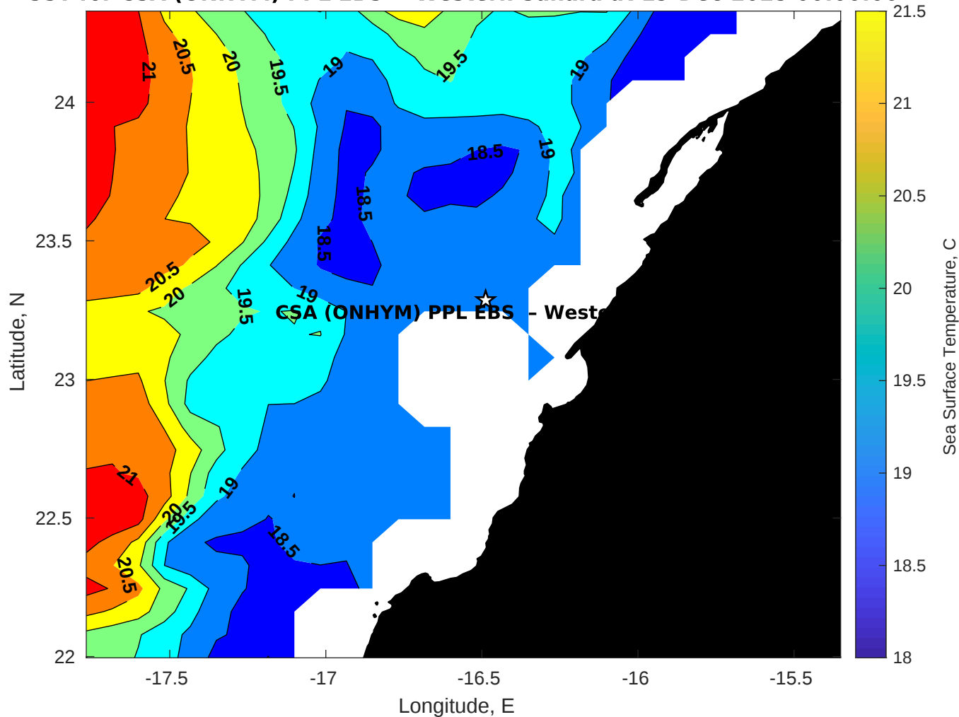
SST for CSA (ONHYM) PPL EBS - Western Sahara at 19-Dec-2025 00:00:00
