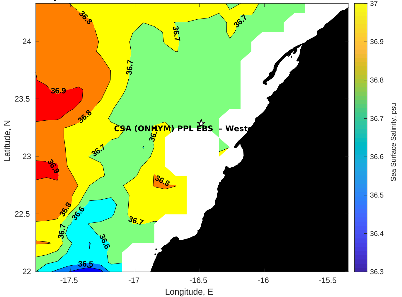
Surface Salinity for CSA (ONHYM) PPL EBS - Western Sahara at 19-Dec-2025 00:00:00
