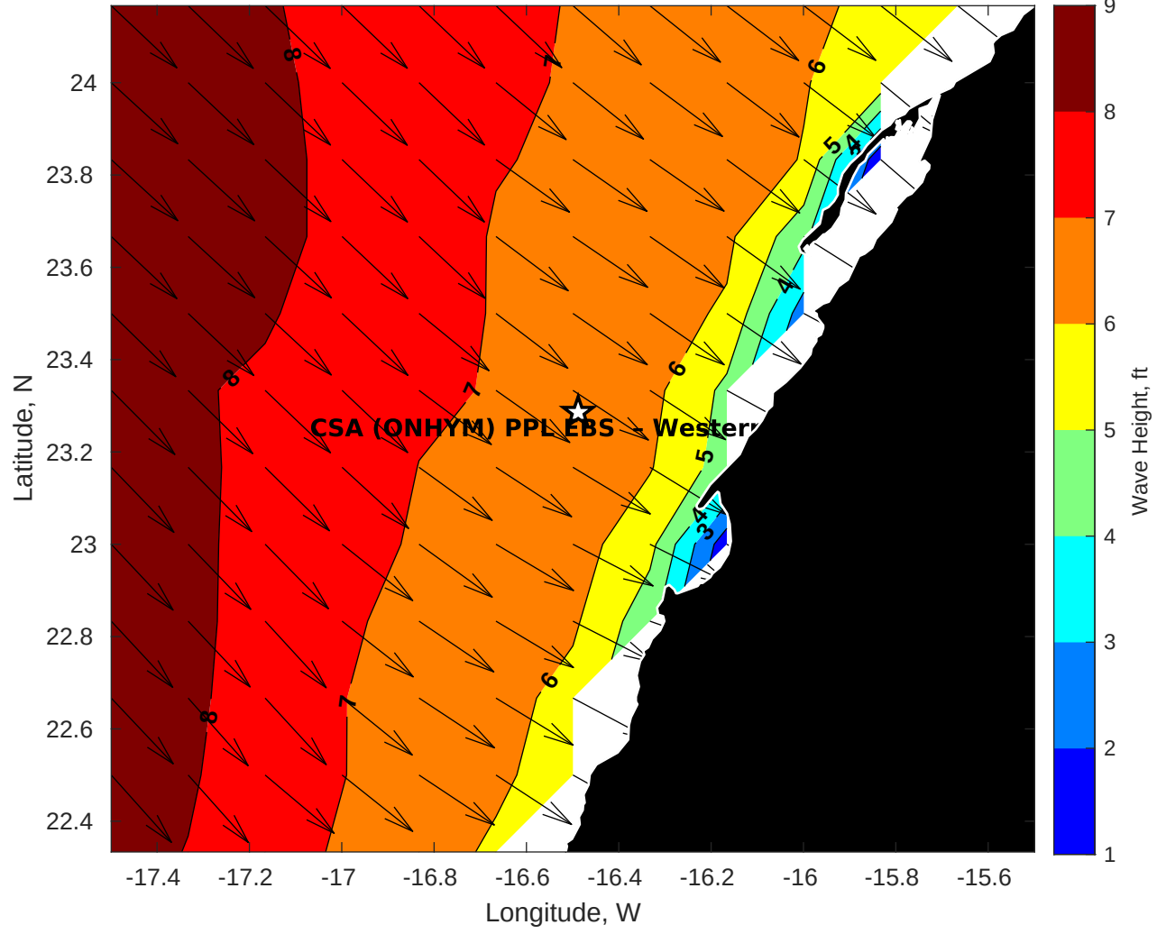
GFS Wave Height (ft) for CSA (ONHYM) PPL EBS - Western Sahara at 20-Dec-2025 09:00:00
