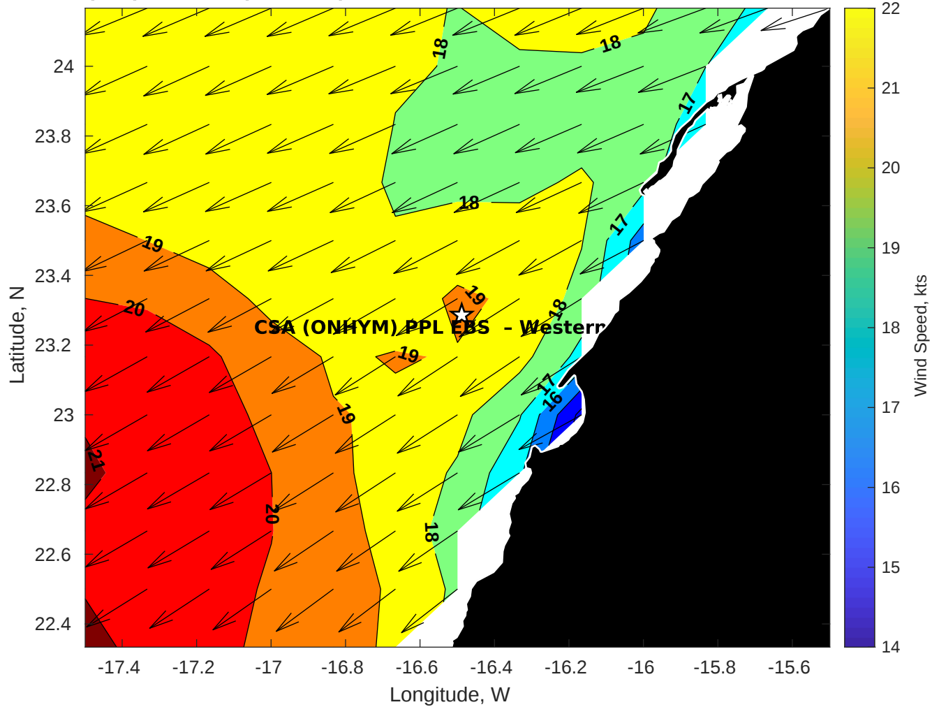
GFS Winds (kts) for CSA (ONHYM) PPL EBS - Western Sahara at 20-Dec-2025 09:00:00
