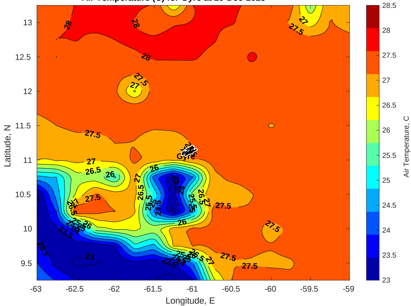
Air Temperature (C) for Gyre at 20-Dec-2025
