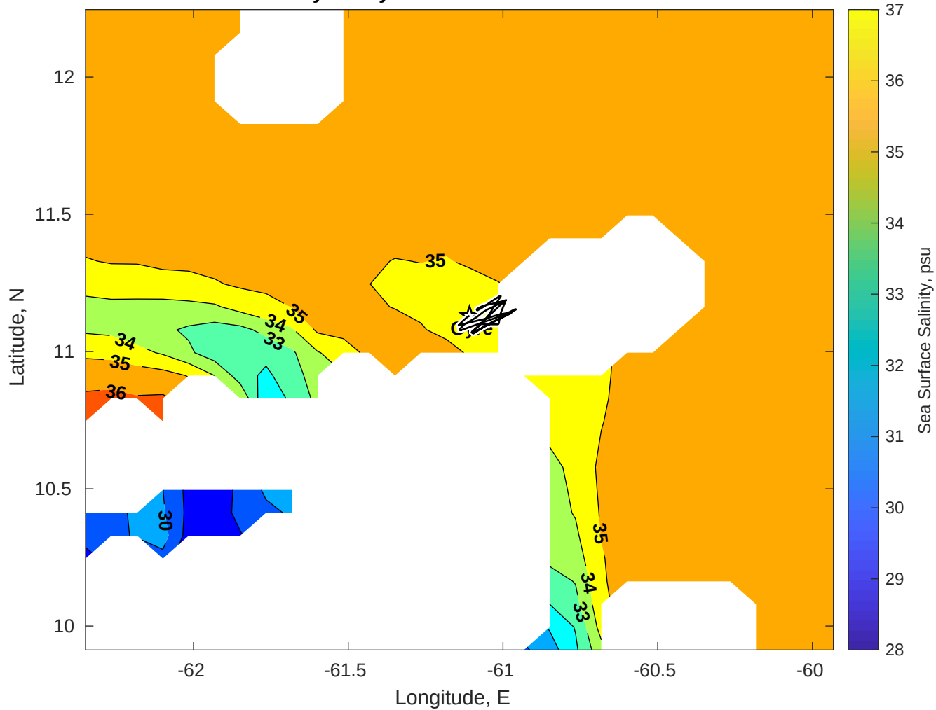
Surface Salinity for Gyre at 19-Dec-2025 00:00:00
