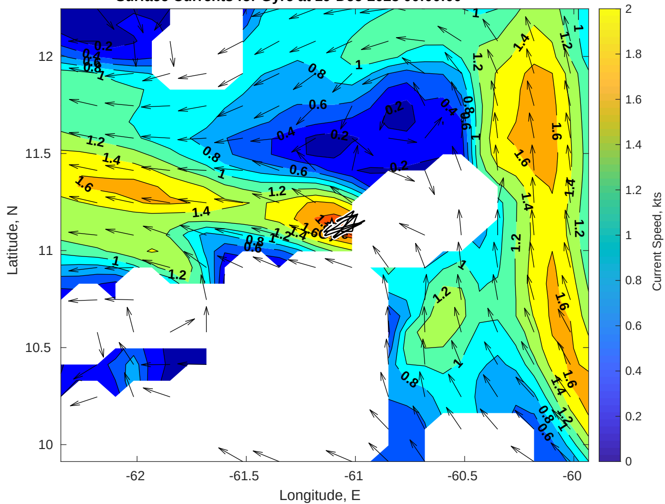
Surface Currents for Gyre at 19-Dec-2025 00:00:00
