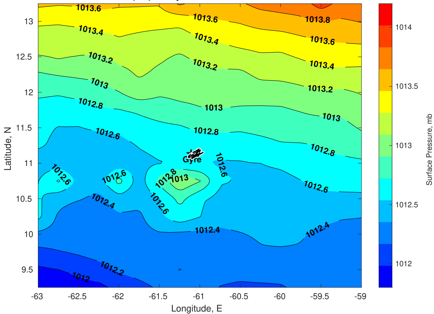
Surface Pressure (mb) for Gyre at 20-Dec-2025 00:00:00
