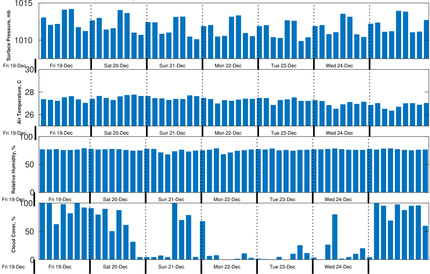
Met Forecast for Gyre from 19-Dec-2025 20:00:00 to 26-Dec-2025 20:00:00
