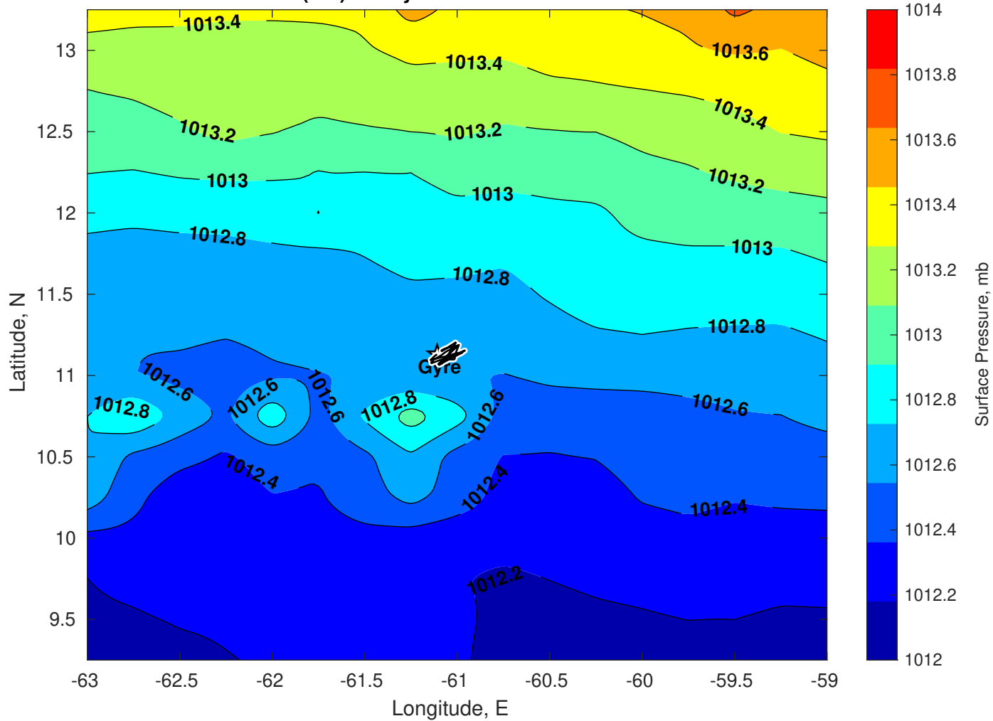
Surface Pressure (mb) for Gyre at 21-Dec-2025 00:00:00
