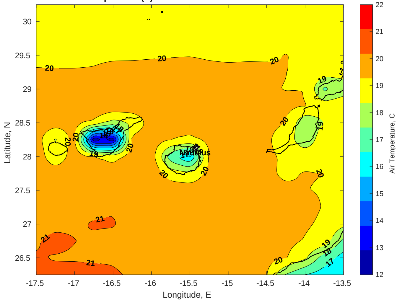
Air Temperature (C) for Nautilus at 20-Dec-2025
