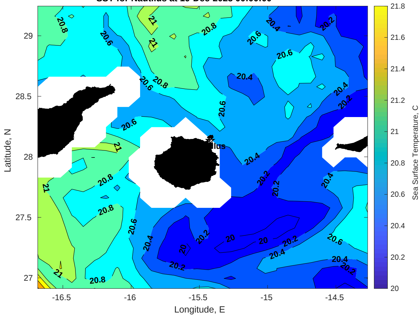
SST for Nautilus at 19-Dec-2025 00:00:00
