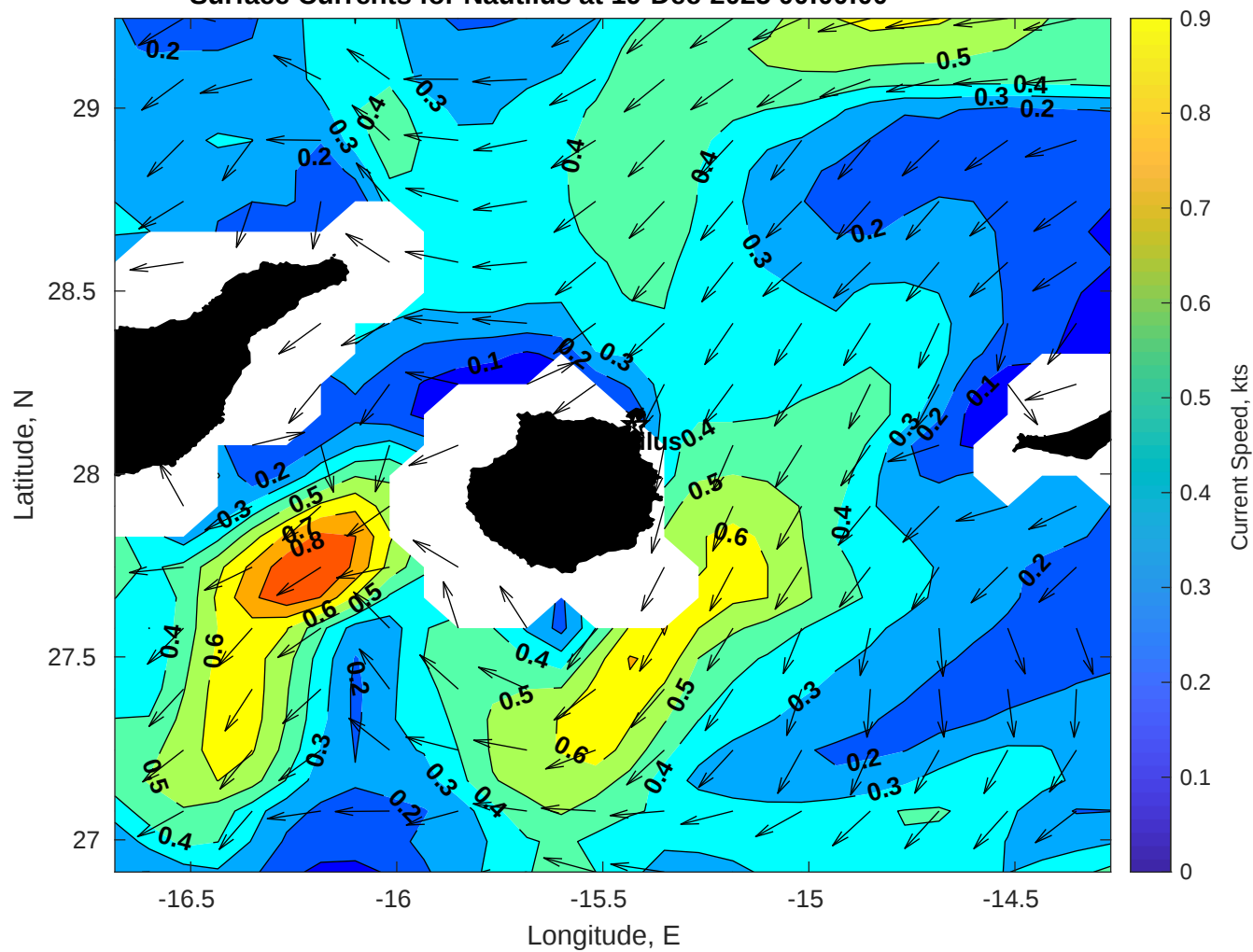
Surface Currents for Nautilus at 19-Dec-2025 00:00:00
