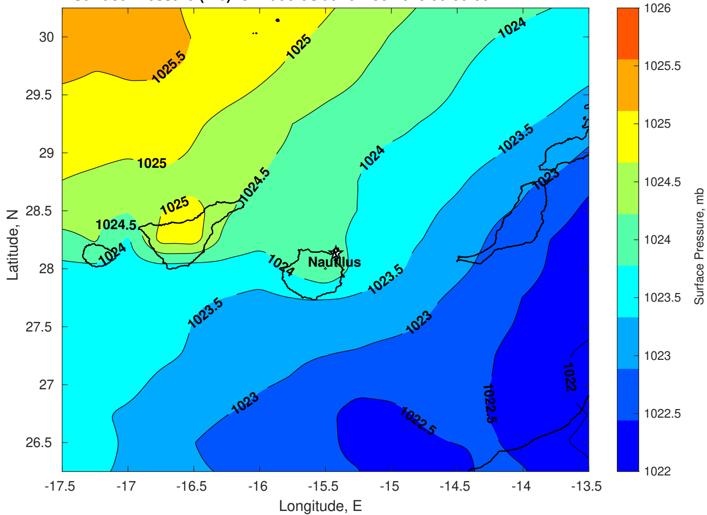
Surface Pressure (mb) for Nautilus at 20-Dec-2025 00:00:00
