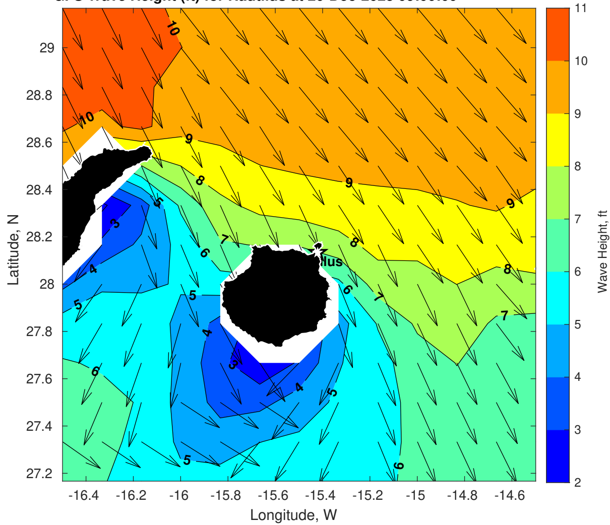
GFS Wave Height (ft) for Nautilus at 20-Dec-2025 09:00:00
