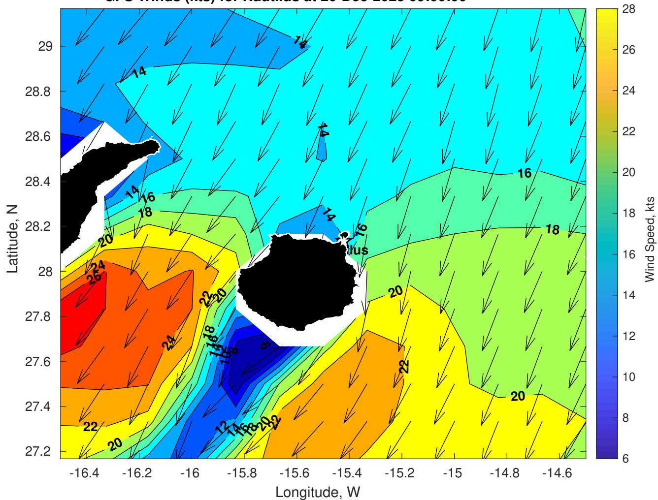
GFS Winds (kts) for Nautilus at 20-Dec-2025 09:00:00
