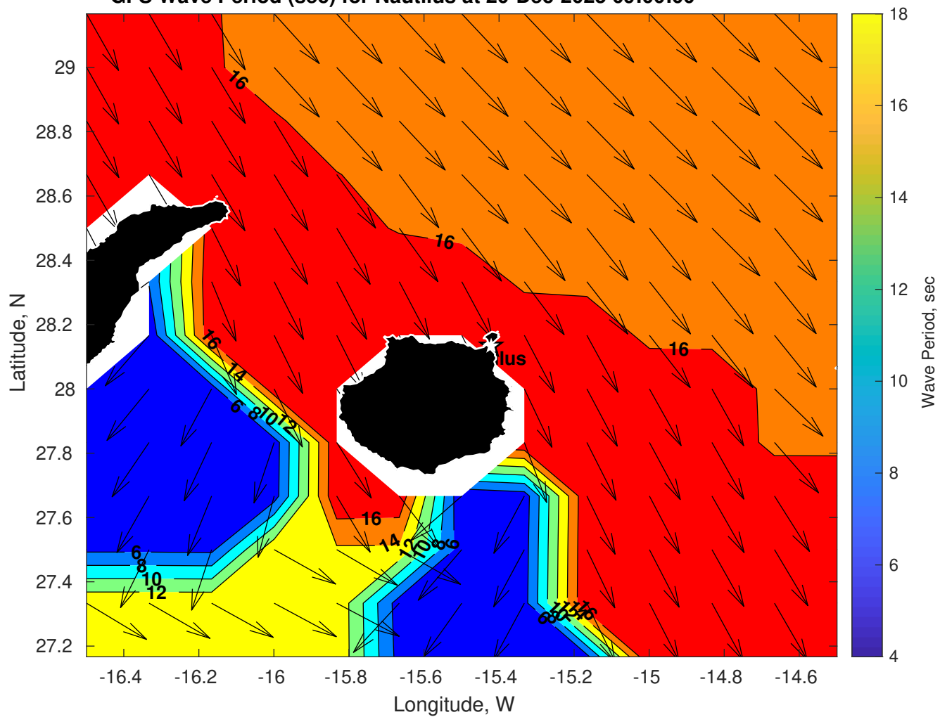
GFS Wave Period (sec) for Nautilus at 20-Dec-2025 09:00:00
