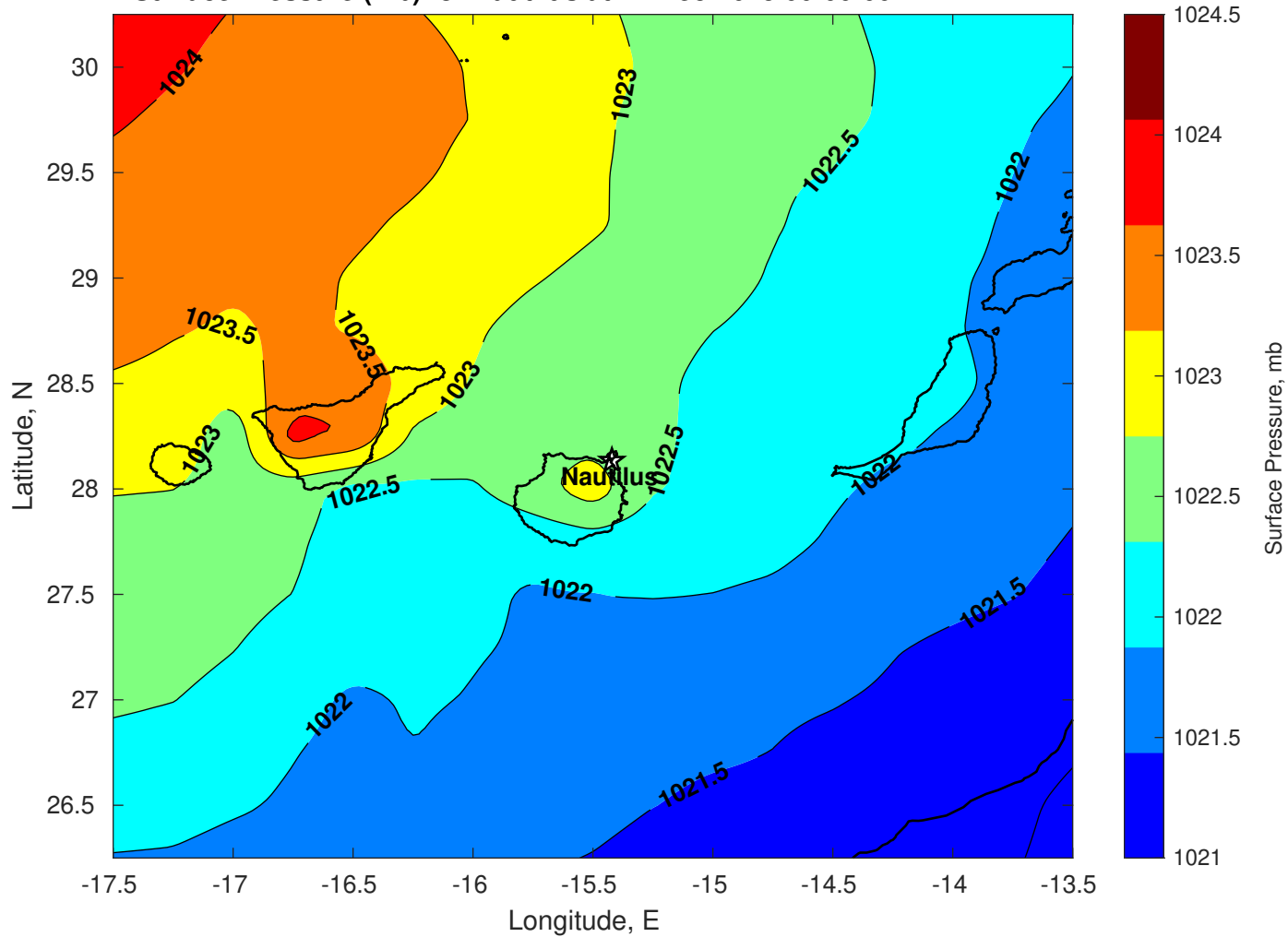
Surface Pressure (mb) for Nautilus at 21-Dec-2025 00:00:00
