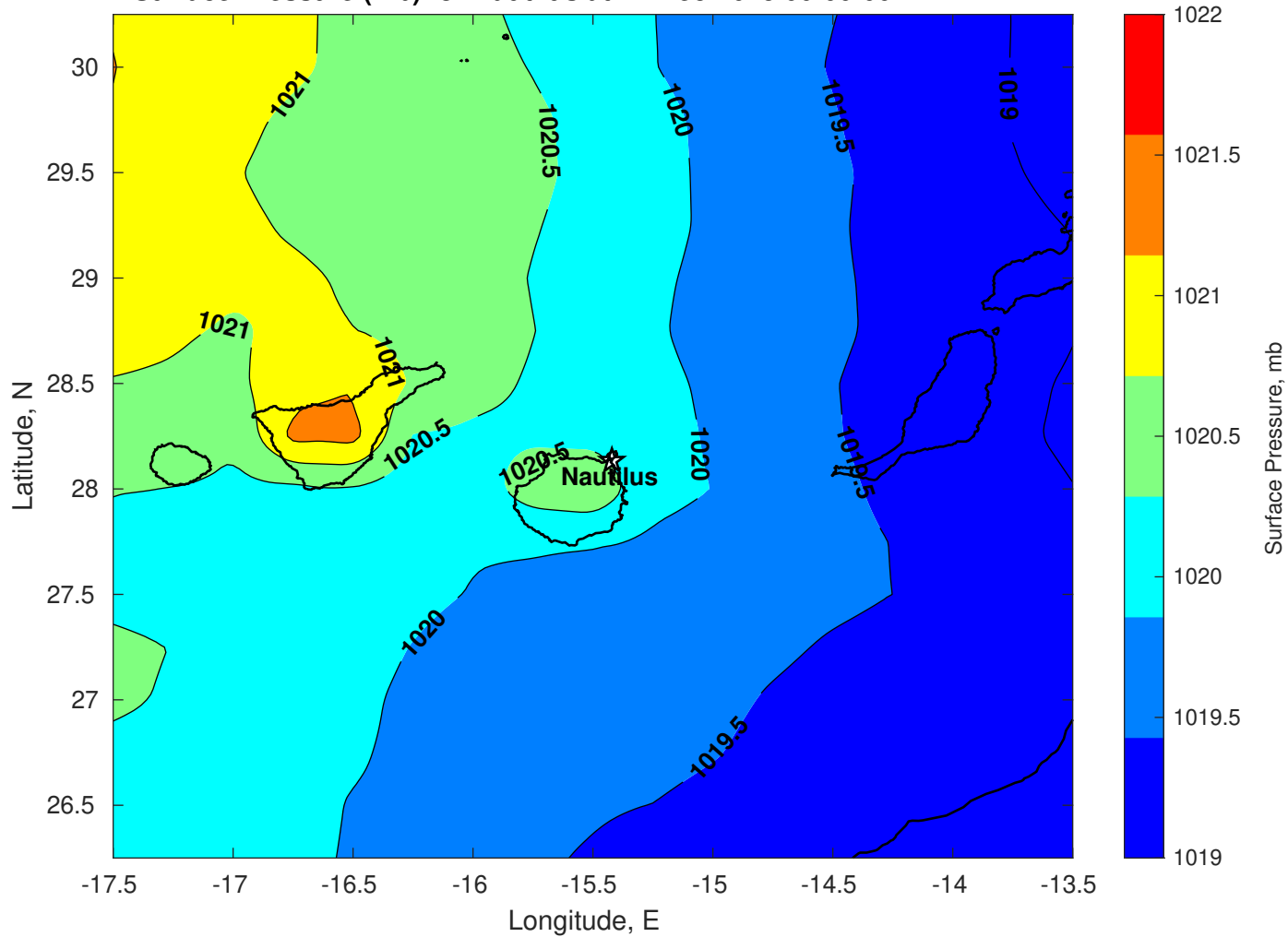
Surface Pressure (mb) for Nautilus at 22-Dec-2025 00:00:00
