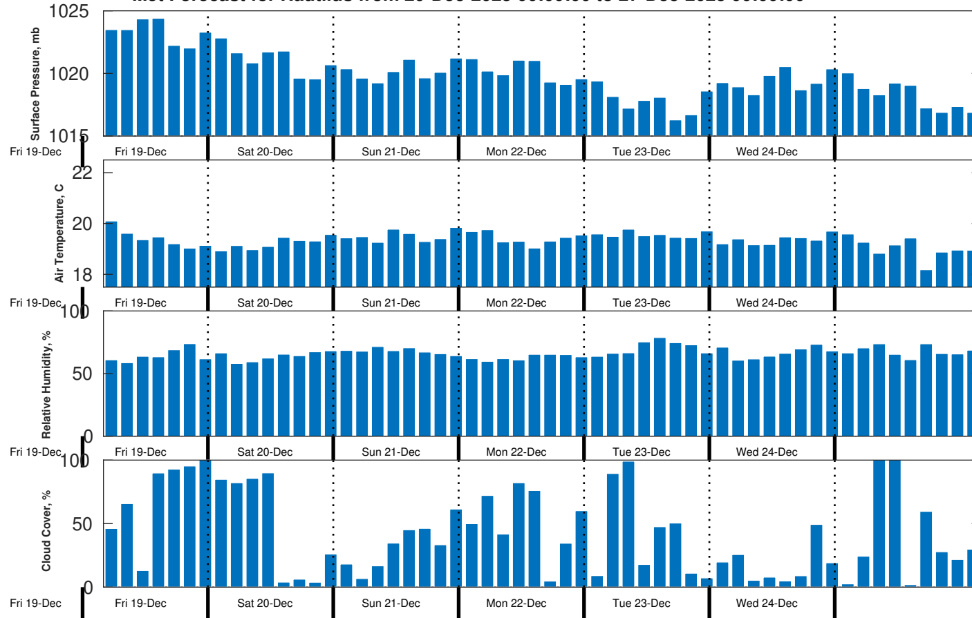
Met Forecast for Nautilus from 20-Dec-2025 00:00:00 to 27-Dec-2025 00:00:00
