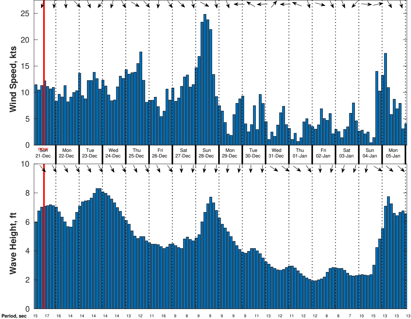
Wind & Wave Forecast for Nautilus from 20-Dec-2025 02:00:00 to 05-Jan-2026 02:00:00
