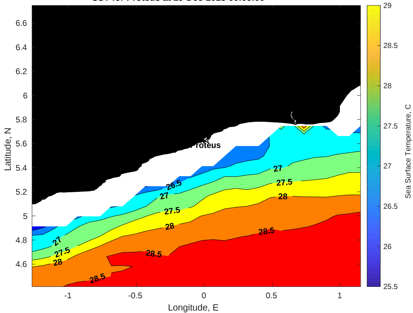
SST for Proteus at 19-Dec-2025 00:00:00
