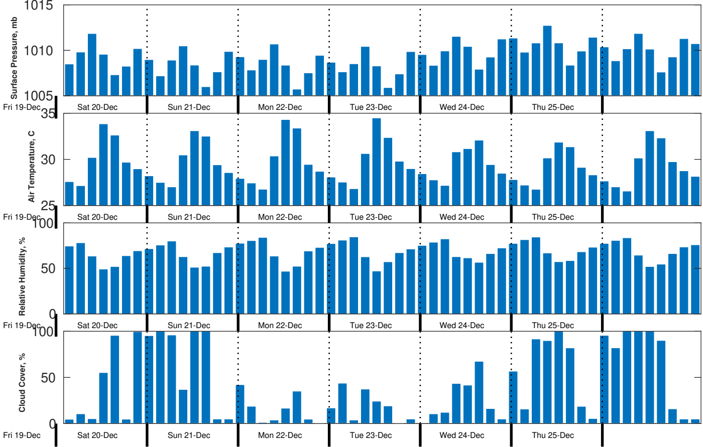
Met Forecast for Proteus from 20-Dec-2025 00:00:00 to 27-Dec-2025 00:00:00
