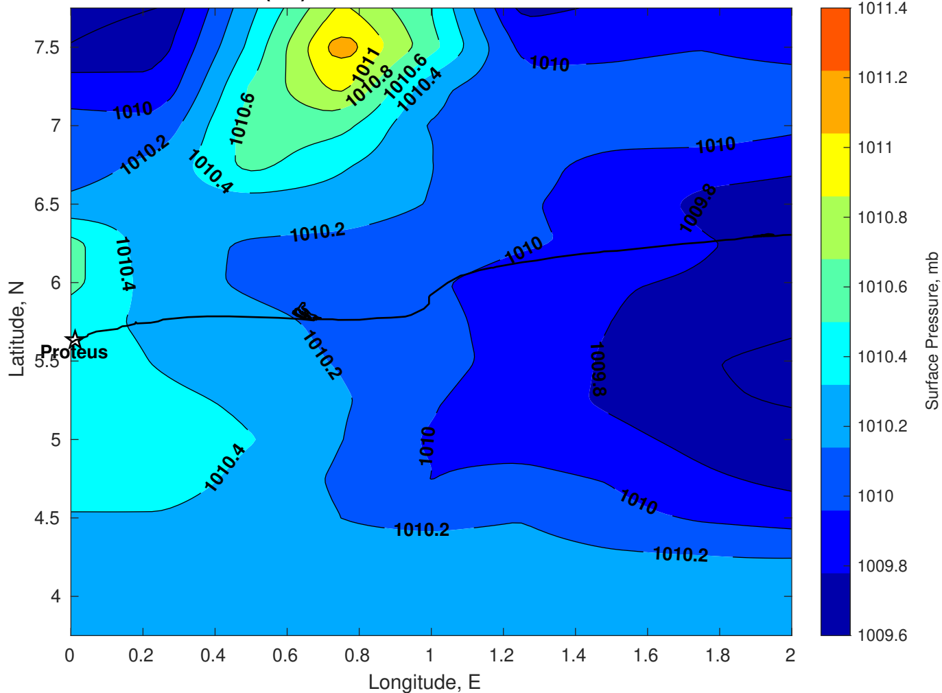
Surface Pressure (mb) for Proteus at 20-Dec-2025 00:00:00
