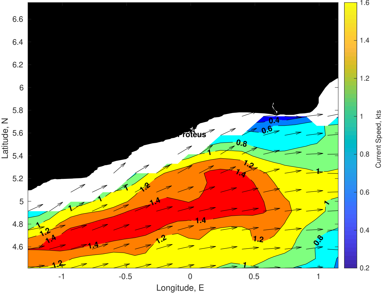
Surface Currents for Proteus at 19-Dec-2025 00:00:00
