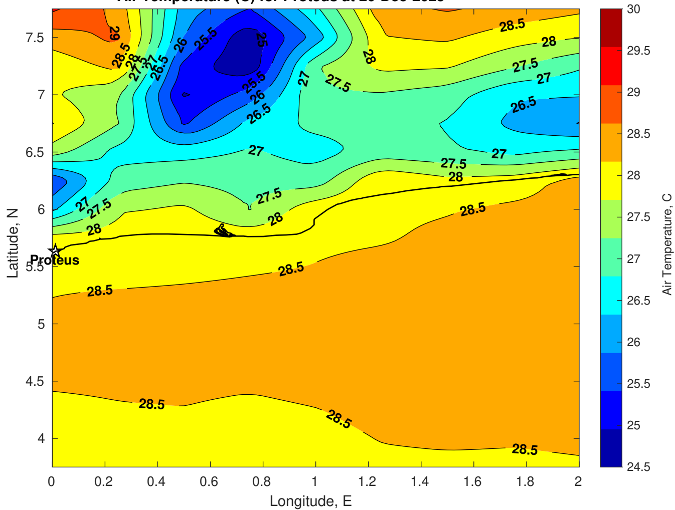
Air Temperature (C) for Proteus at 20-Dec-2025
