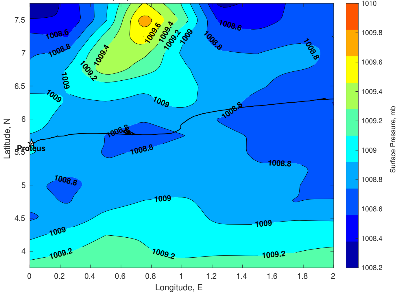
Surface Pressure (mb) for Proteus at 21-Dec-2025 00:00:00
