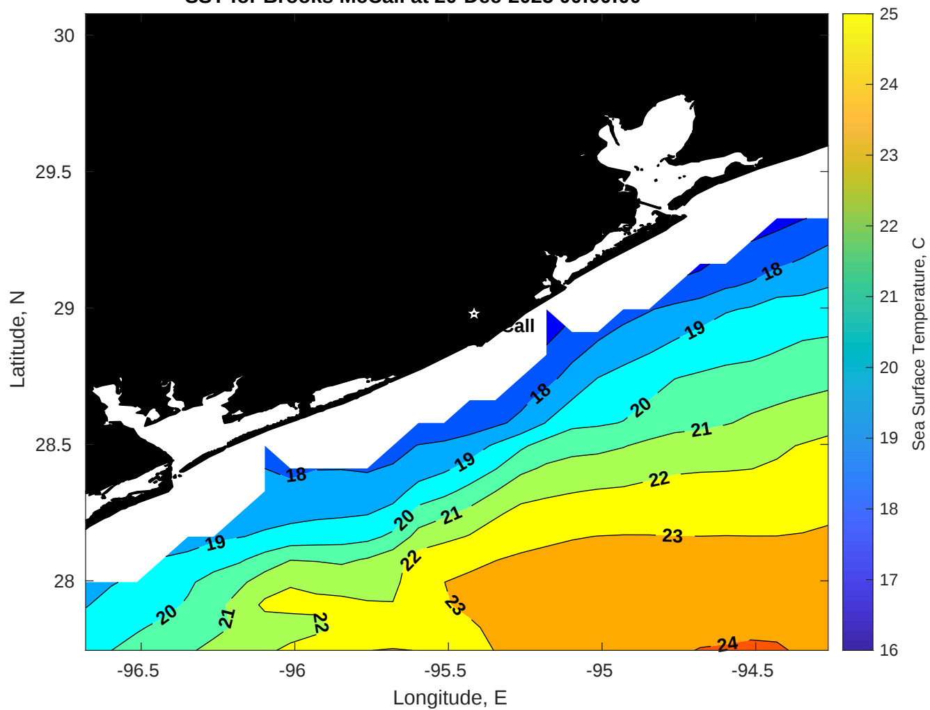
SST for Brooks McCall at 20-Dec-2025 00:00:00
