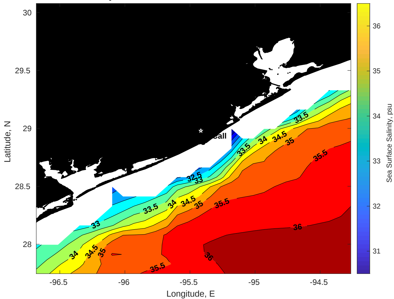
Surface Salinity for Brooks McCall at 20-Dec-2025 00:00:00
