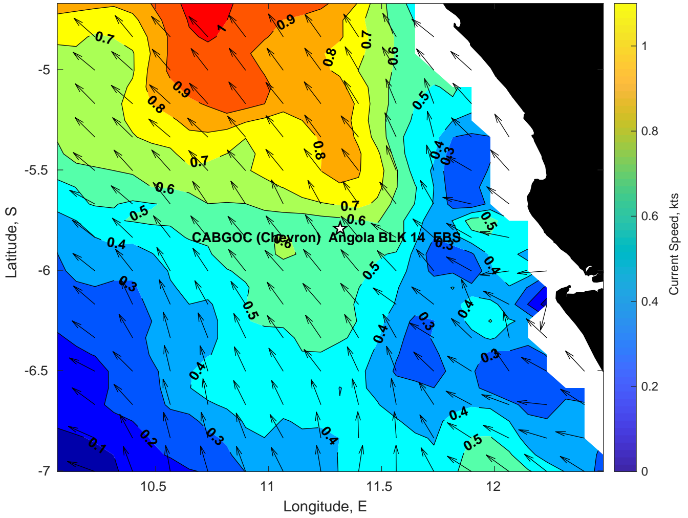
Surface Currents for CABGOC (Chevron) Angola BLK 14 EBS at 13-Jul-2025 00:00:00
