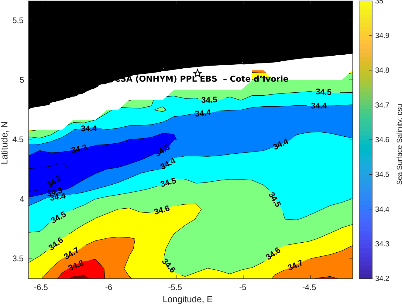
Surface Salinity for CSA (ONHYM) PPL EBS - Cote d'Ivoire at 20-Dec-2025 00:00:00
