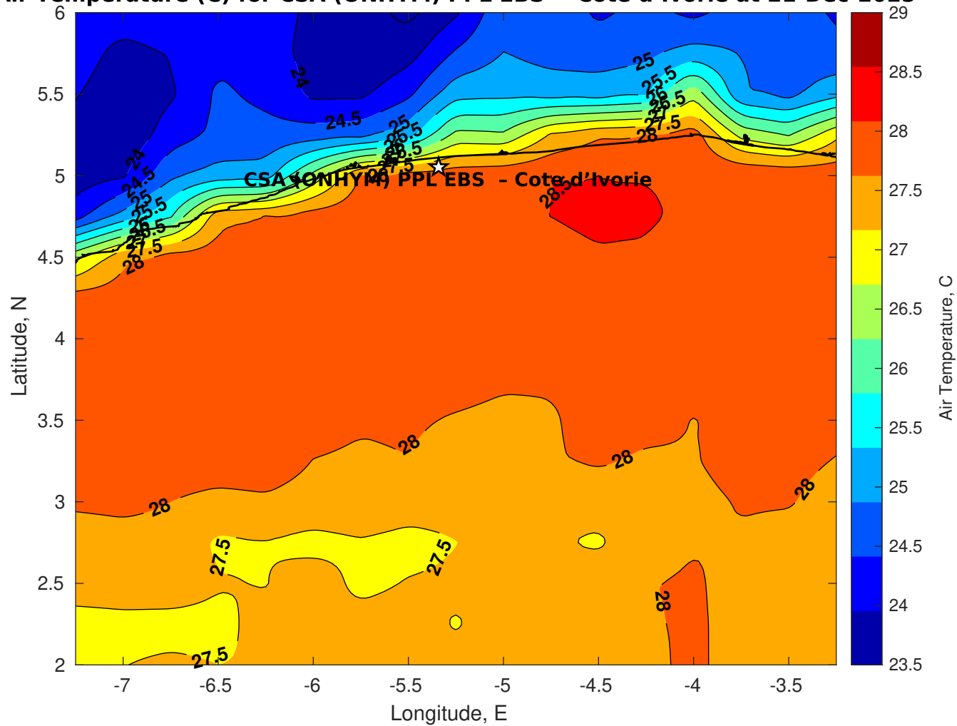
Air Temperature (C) for CSA (ONHYM) PPL EBS - Cote d'Ivoire at 21-Dec-2025
