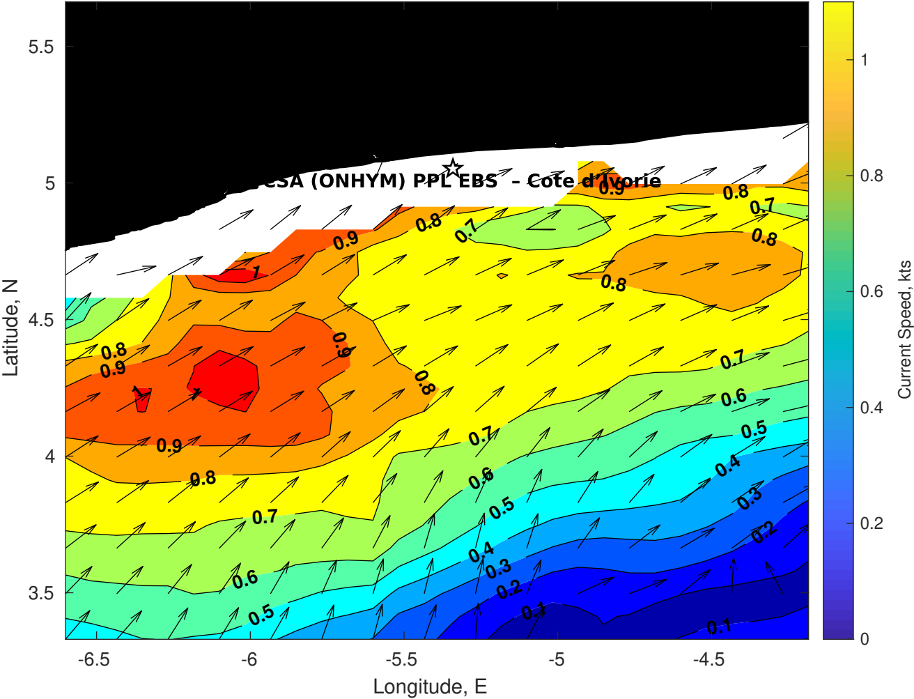
Surface Currents for CSA (ONHYM) PPL EBS - Cote d'Ivoire at 20-Dec-2025 00:00:00
