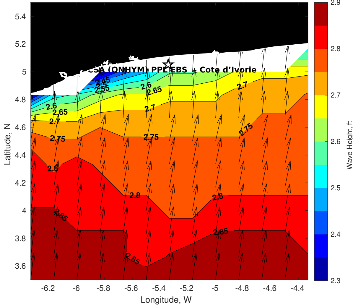
GFS Wave Height (ft) for CSA (ONHYM) PPL EBS - Cote d'Ivoire at 21-Dec-2025 09:00:00
