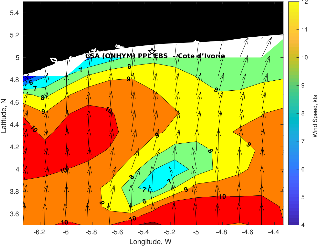
GFS Winds (kts) for CSA (ONHYM) PPL EBS - Cote d'Ivoire at 21-Dec-2025 09:00:00
