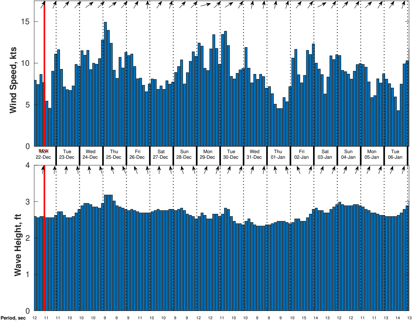
Wind & Wave Forecast for CSA (ONHYM) PPL EBS - Cote d'Ivoire from 21-Dec-2025 01:00:00 to 06-Jan-2026 01:00:00
