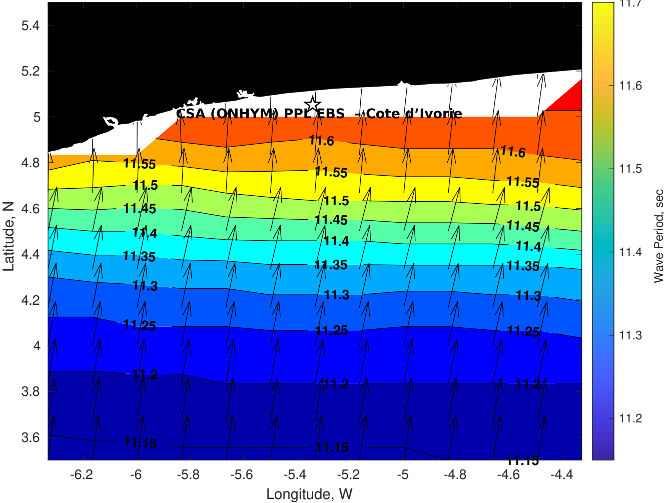
GFS Wave Period (sec) for CSA (ONHYM) PPL EBS - Cote d'Ivoire at 21-Dec-2025 09:00:00
