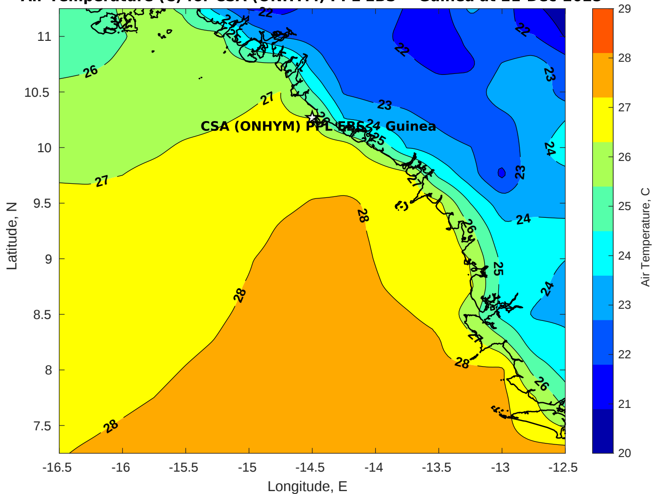
Air Temperature (C) for CSA (ONHYM) PPL EBS - Guinea at 21-Dec-2025
