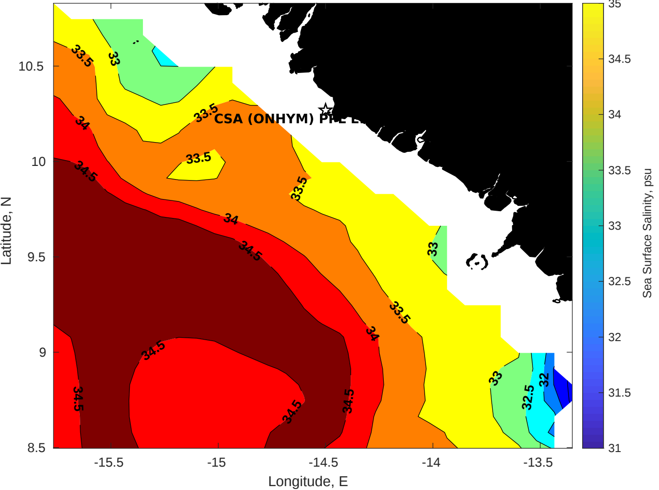
Surface Salinity for CSA (ONHYM) PPL EBS - Guinea at 20-Dec-2025 00:00:00
