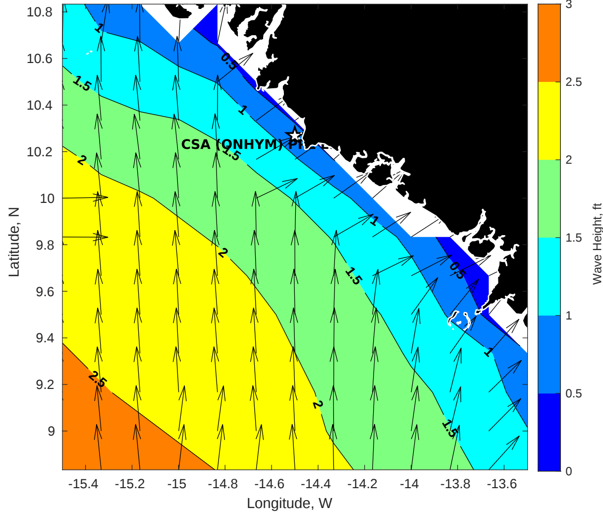
GFS Wave Height (ft) for CSA (ONHYM) PPL EBS - Guinea at 21-Dec-2025 09:00:00
