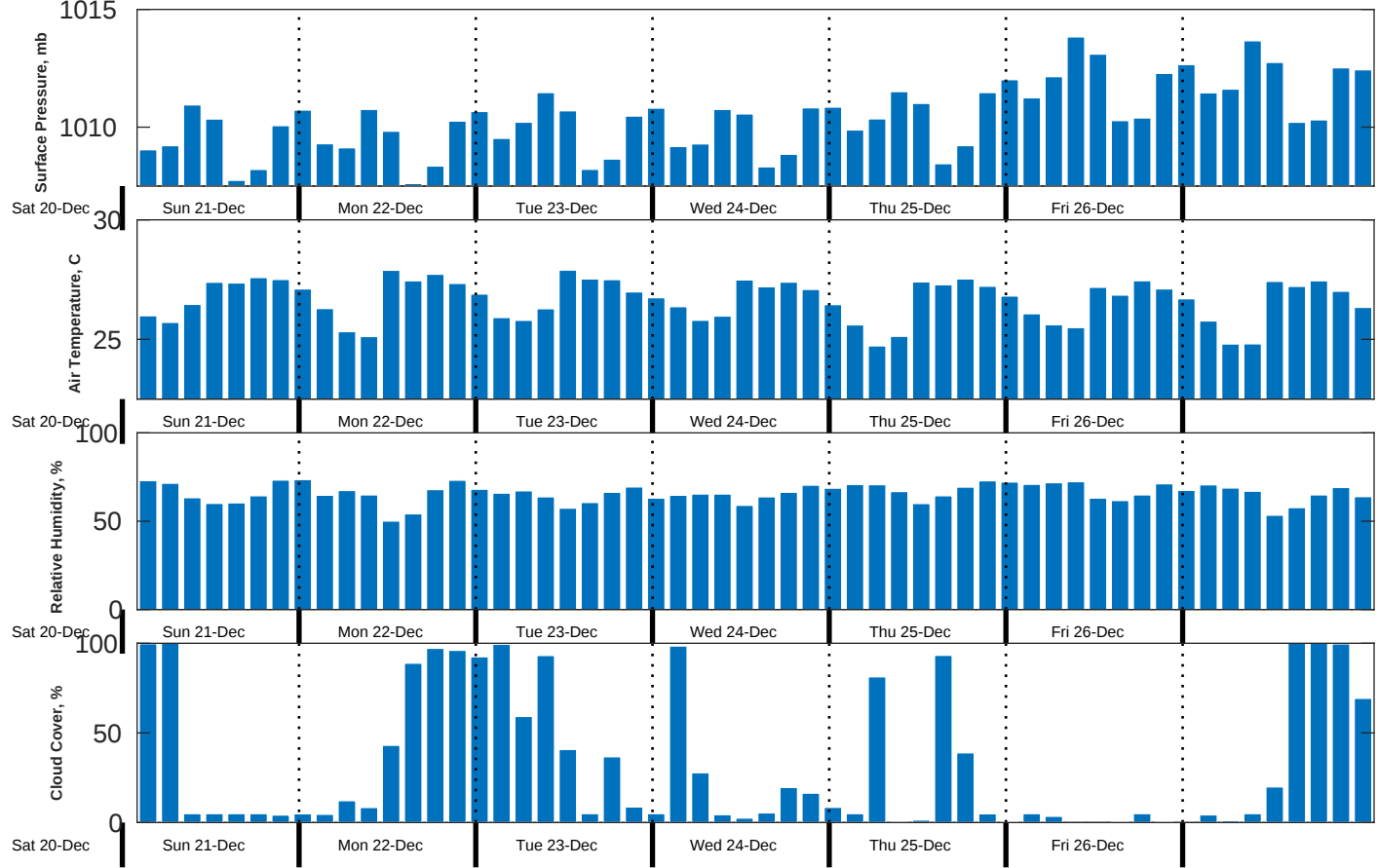
Met Forecast for CSA (ONHYM) PPL EBS - Guinea from 21-Dec-2025 00:00:00 to 28-Dec-2025 00:00:00
