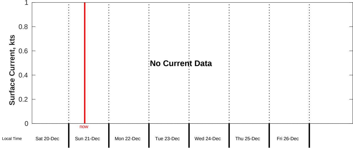
Surface Current Forecast for CSA (ONHYM) PPL EBS - Guinea from 20-Dec-2025 00:00:00 to 28-Dec-2025 00:00:00
