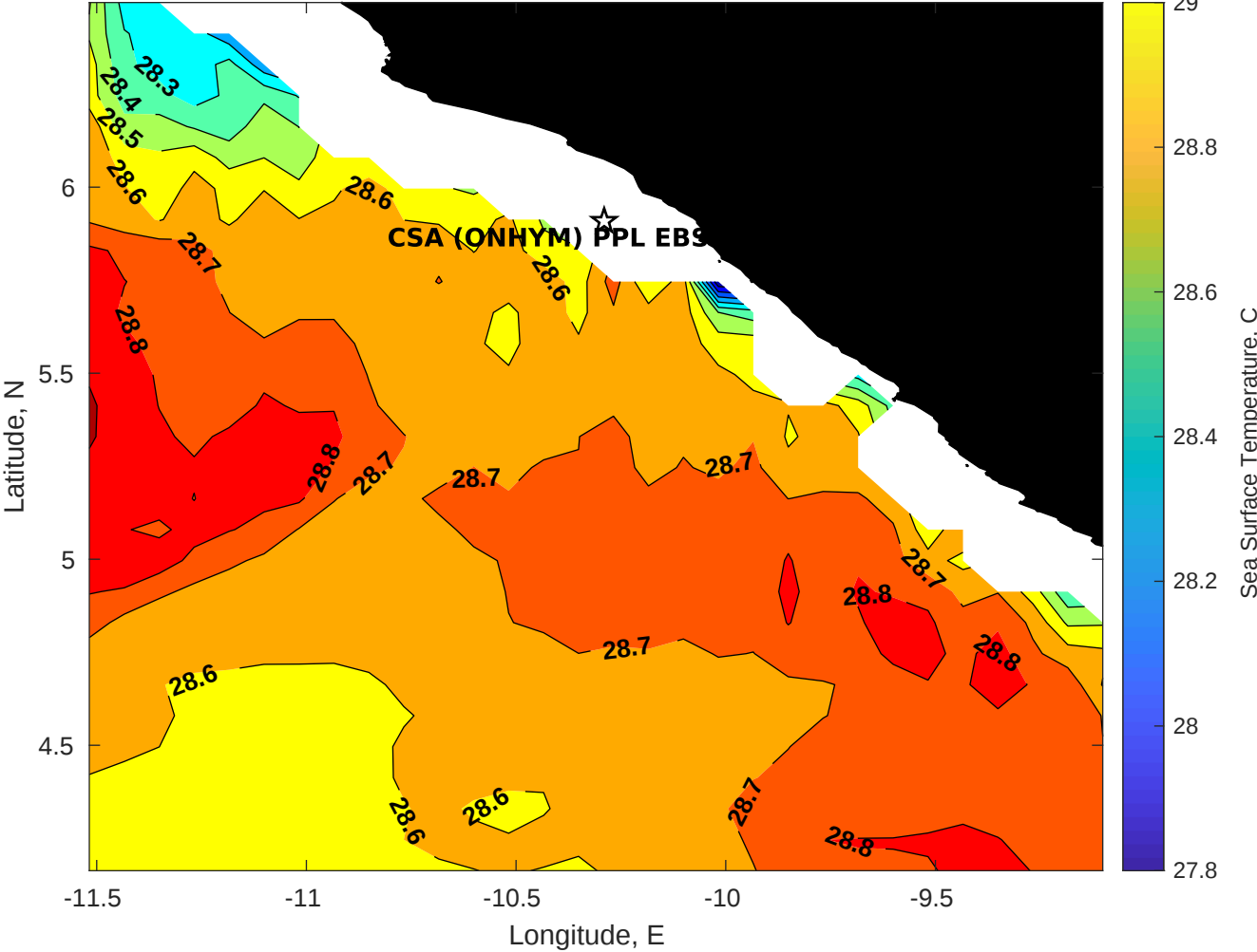
SST for CSA (ONHYM) PPL EBS - Liberia at 20-Dec-2025 00:00:00
