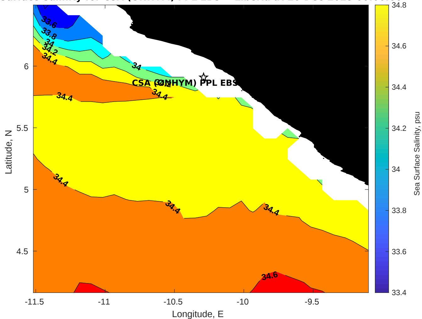
Surface Salinity for CSA (ONHYM) PPL EBS - Liberia at 20-Dec-2025 00:00:00
