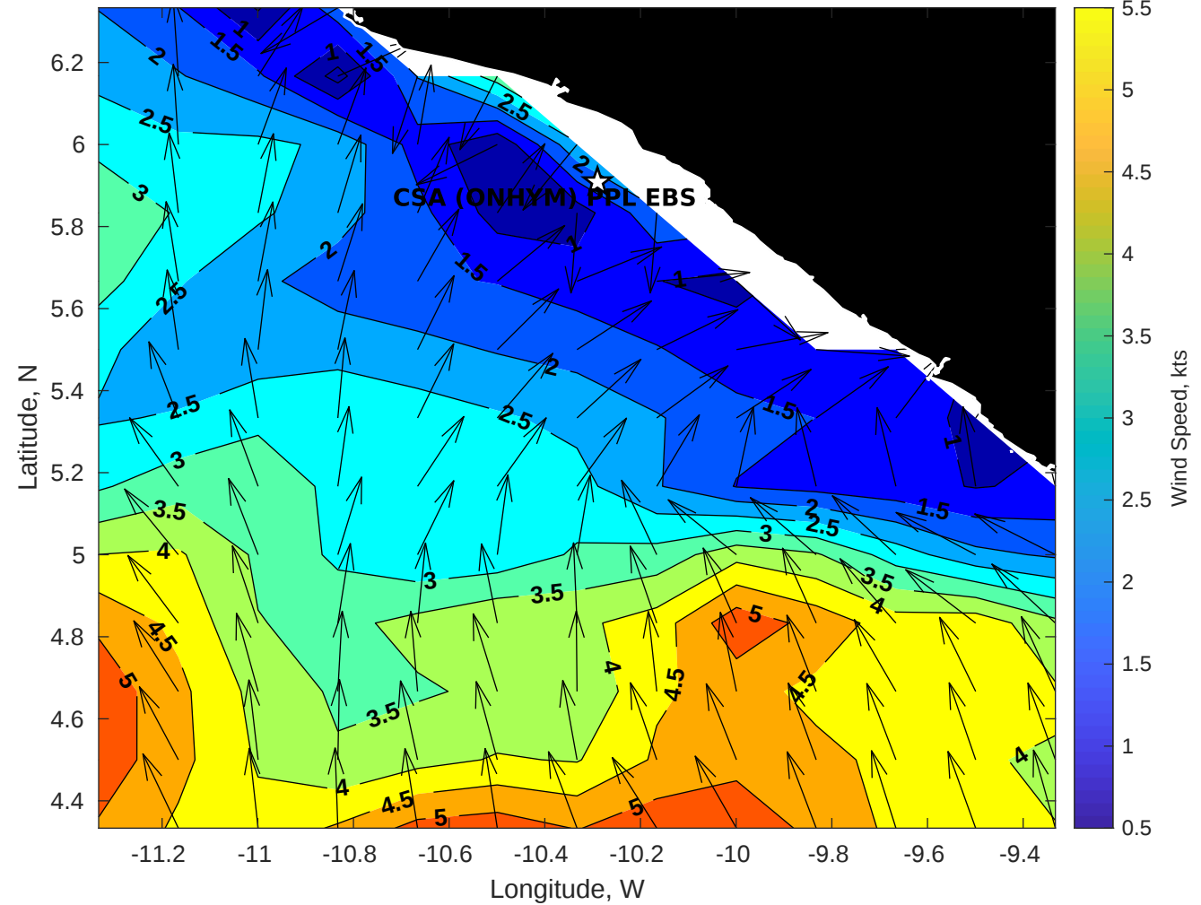
GFS Winds (kts) for CSA (ONHYM) PPL EBS - Liberia at 21-Dec-2025 09:00:00
