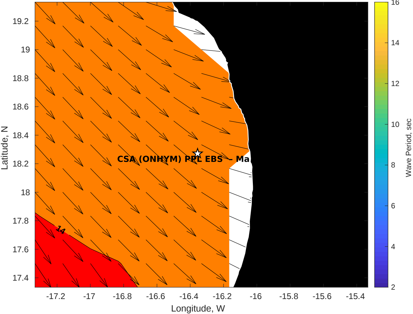
GFS Wave Period (sec) for CSA (ONHYM) PPL EBS - Mauritania at 21-Dec-2025 09:00:00
