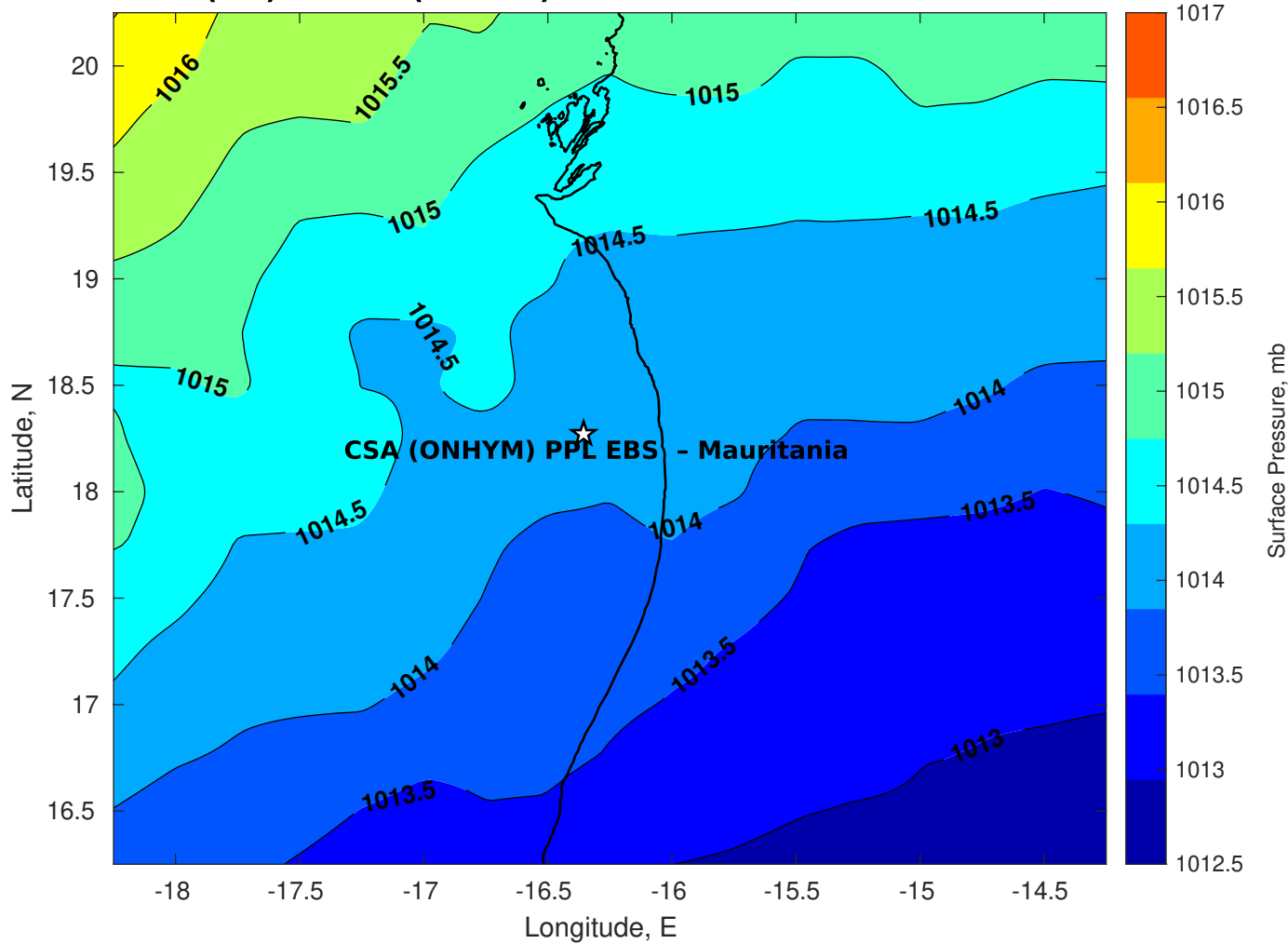
Surface Pressure (mb) for CSA (ONHYM) PPL EBS - Mauritania at 22-Dec-2025 00:00:00
