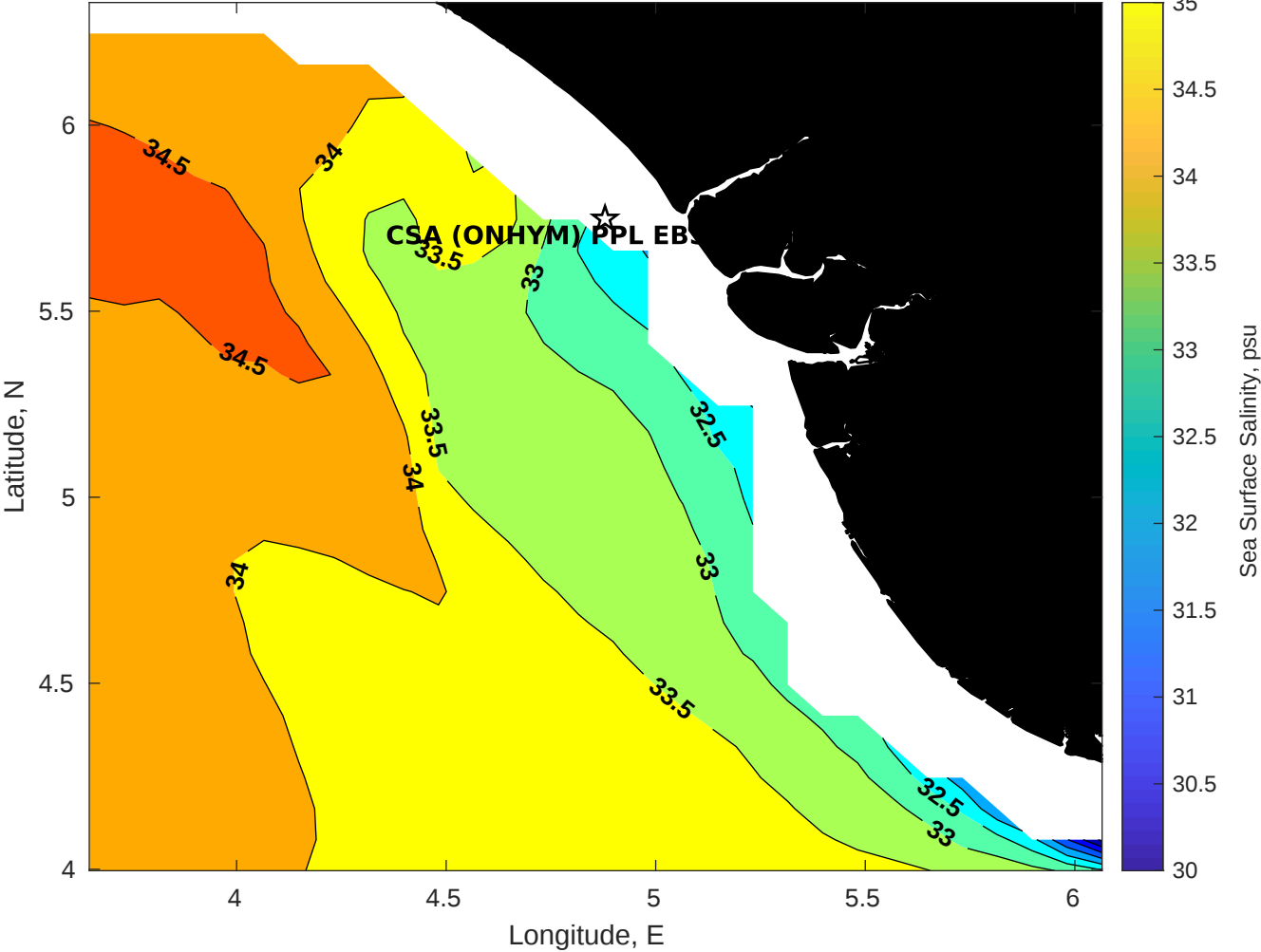
Surface Salinity for CSA (ONHYM) PPL EBS - Nigeria at 20-Dec-2025 00:00:00
