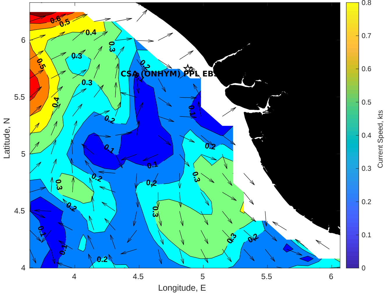
Surface Currents for CSA (ONHYM) PPL EBS - Nigeria at 20-Dec-2025 00:00:00
