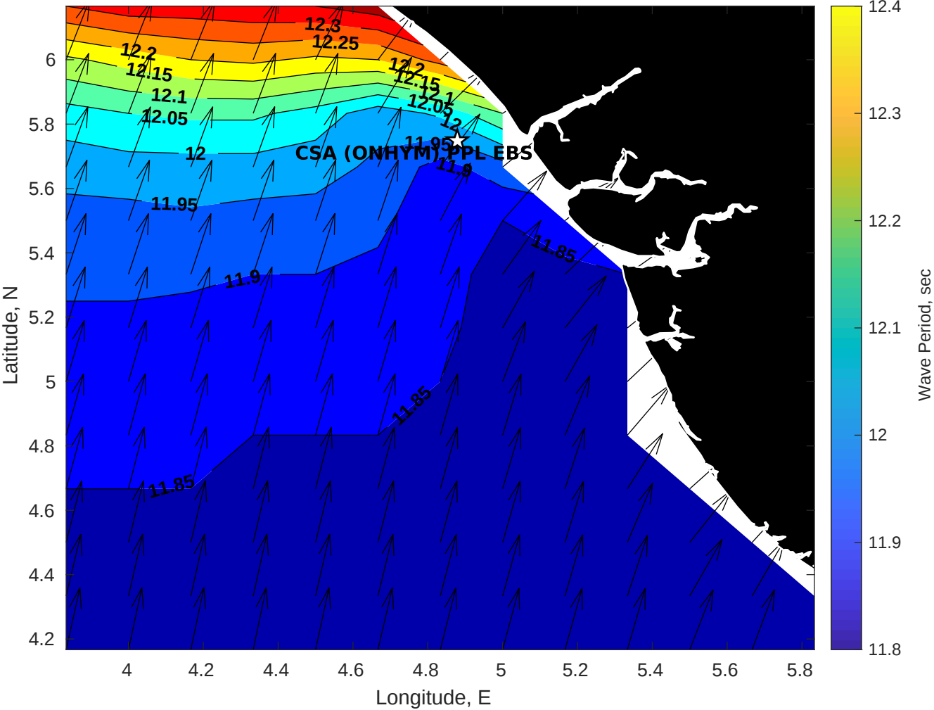
GFS Wave Period (sec) for CSA (ONHYM) PPL EBS - Nigeria at 21-Dec-2025 09:00:00
