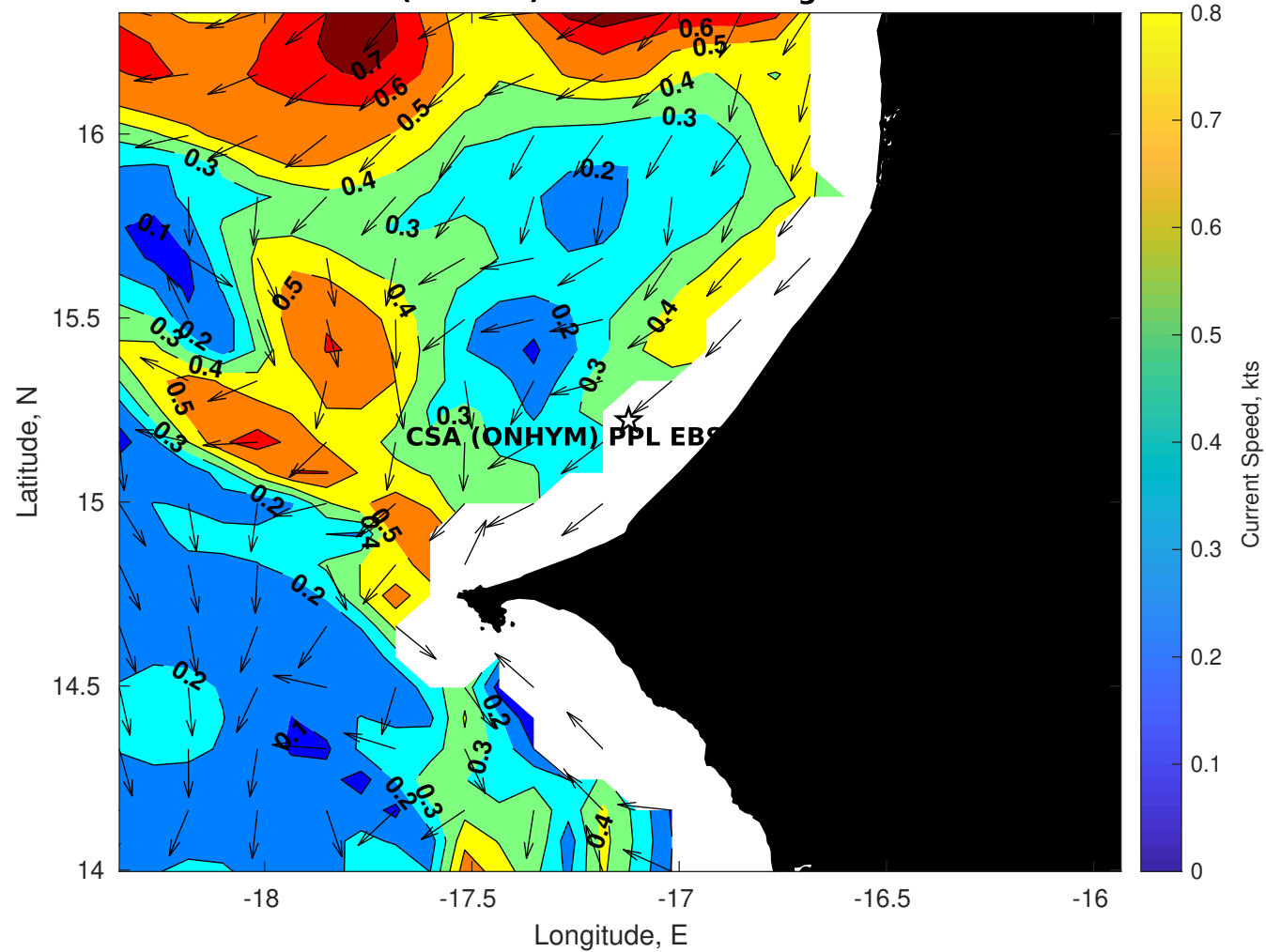
Surface Currents for CSA (ONHYM) PPL EBS - Senegal at 20-Dec-2025 00:00:00
