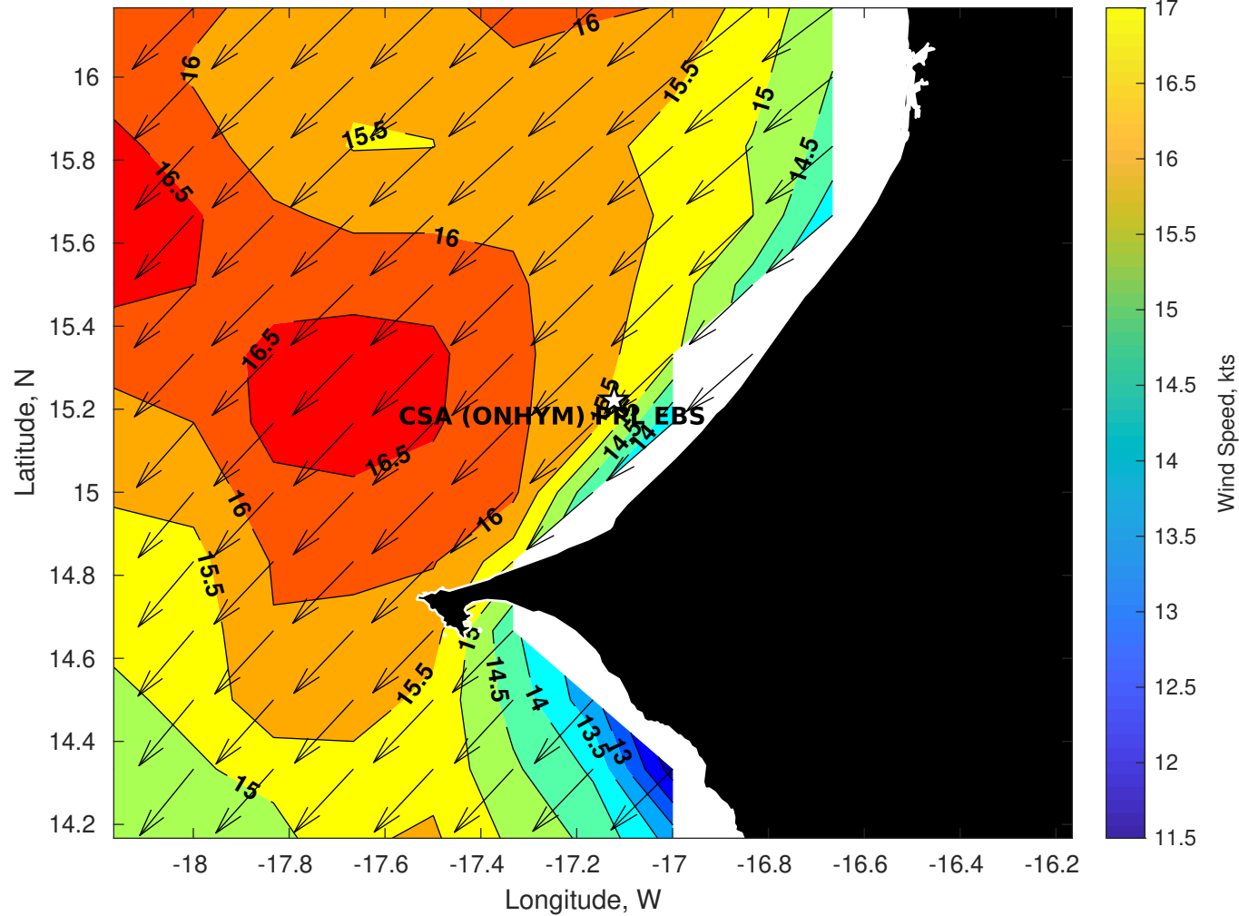
GFS Winds (kts) for CSA (ONHYM) PPL EBS - Senegal at 21-Dec-2025 09:00:00
