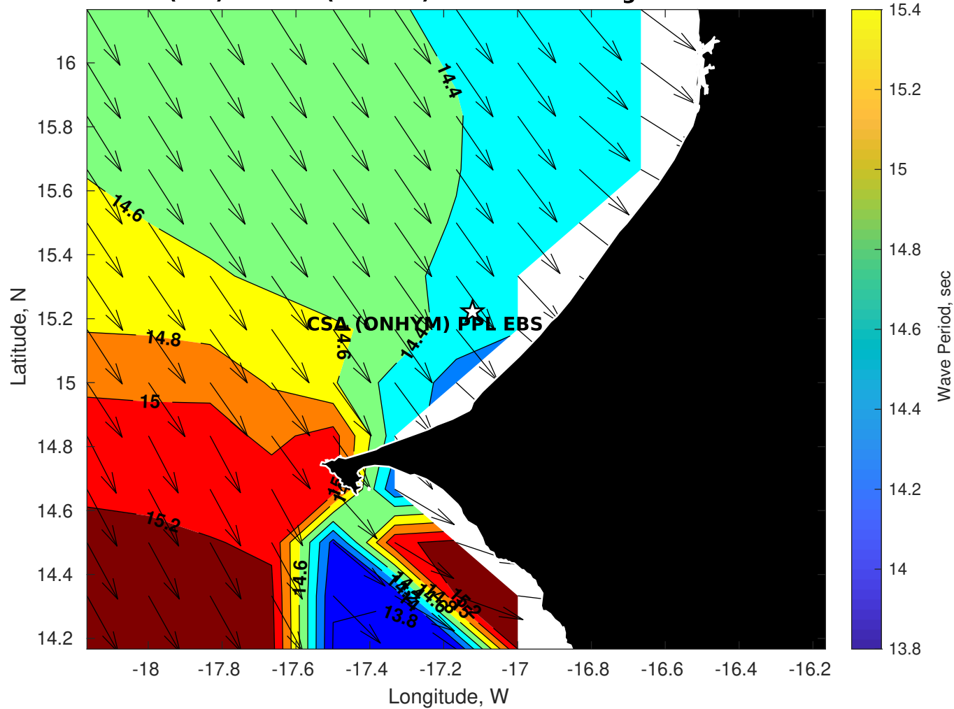
GFS Wave Period (sec) for CSA (ONHYM) PPL EBS - Senegal at 21-Dec-2025 09:00:00
