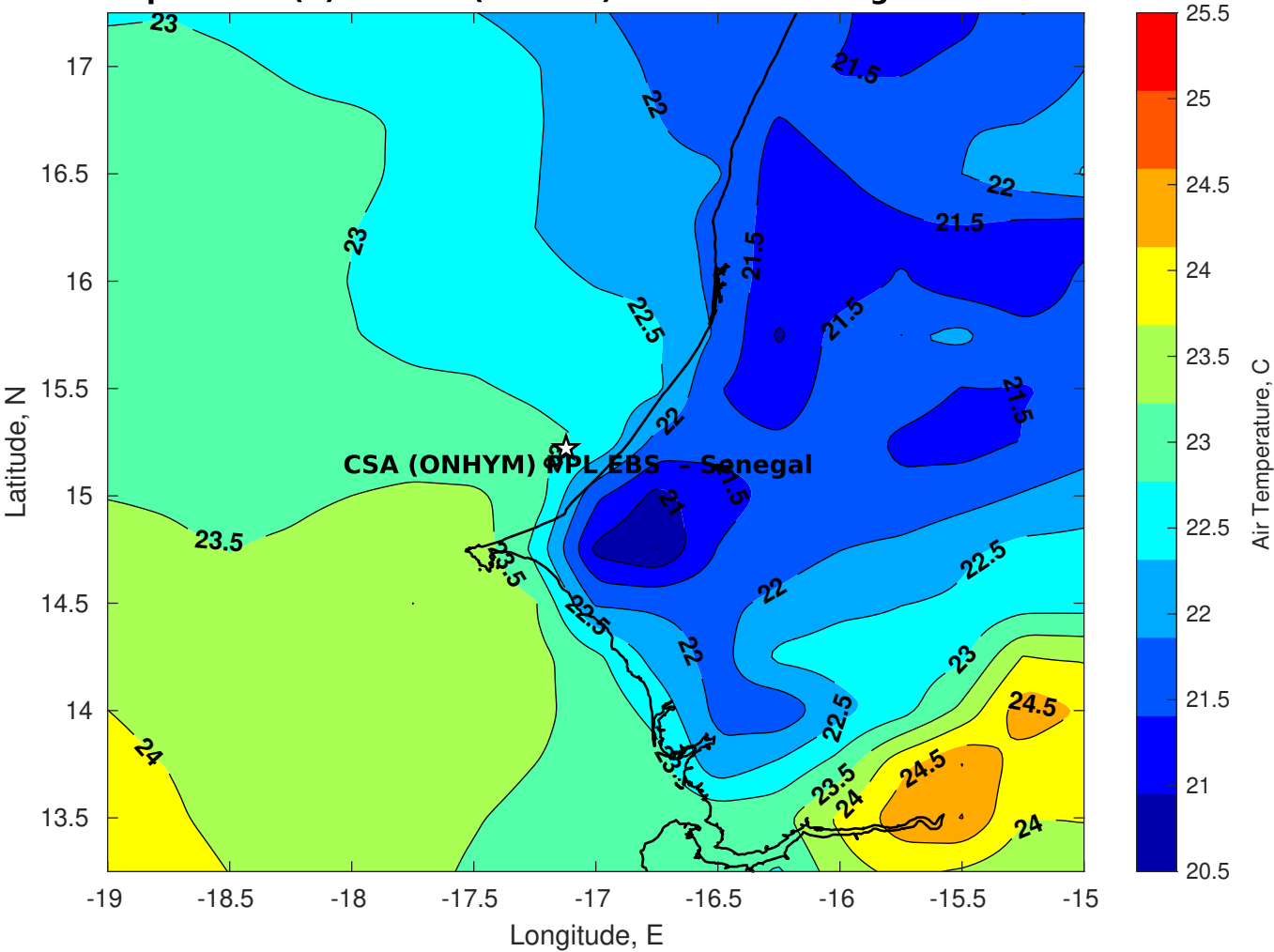
Air Temperature (C) for CSA (ONHYM) PPL EBS - Senegal at 21-Dec-2025
