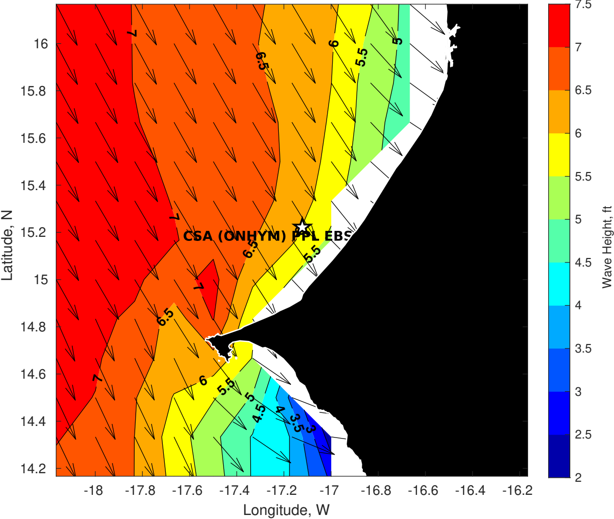
GFS Wave Height (ft) for CSA (ONHYM) PPL EBS - Senegal at 21-Dec-2025 09:00:00
