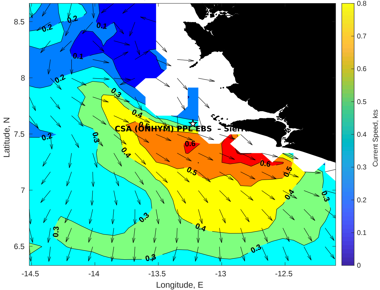
Surface Currents for CSA (ONHYM) PPL EBS - Sierra Leone at 20-Dec-2025 00:00:00
