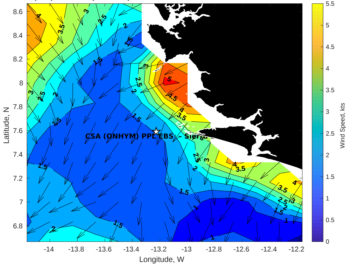
GFS Winds (kts) for CSA (ONHYM) PPL EBS - Sierra Leone at 21-Dec-2025 09:00:00
