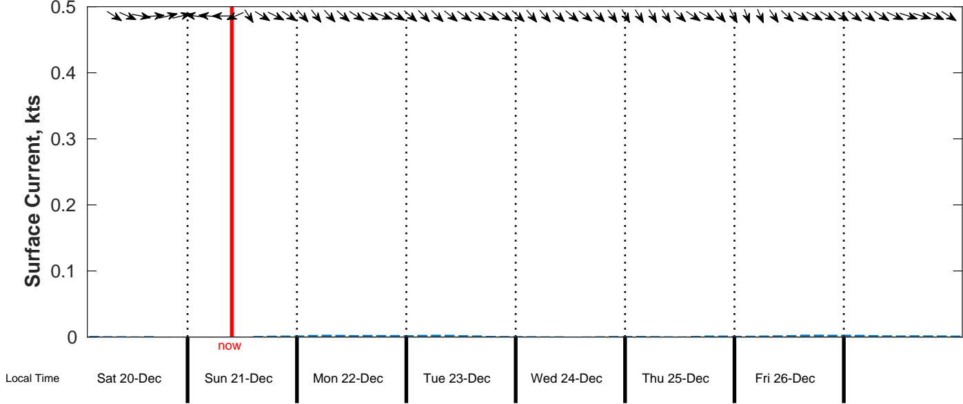
Surface Current Forecast for CSA (ONHYM) PPL EBS - Sierra Leone from 20-Dec-2025 00:00:00 to 28-Dec-2025 00:00:00
