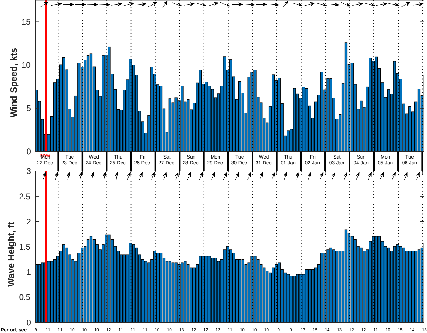
Wind & Wave Forecast for CSA (ONHYM) PPL EBS - Sierra Leone from 21-Dec-2025 01:00:00 to 06-Jan-2026 01:00:00
