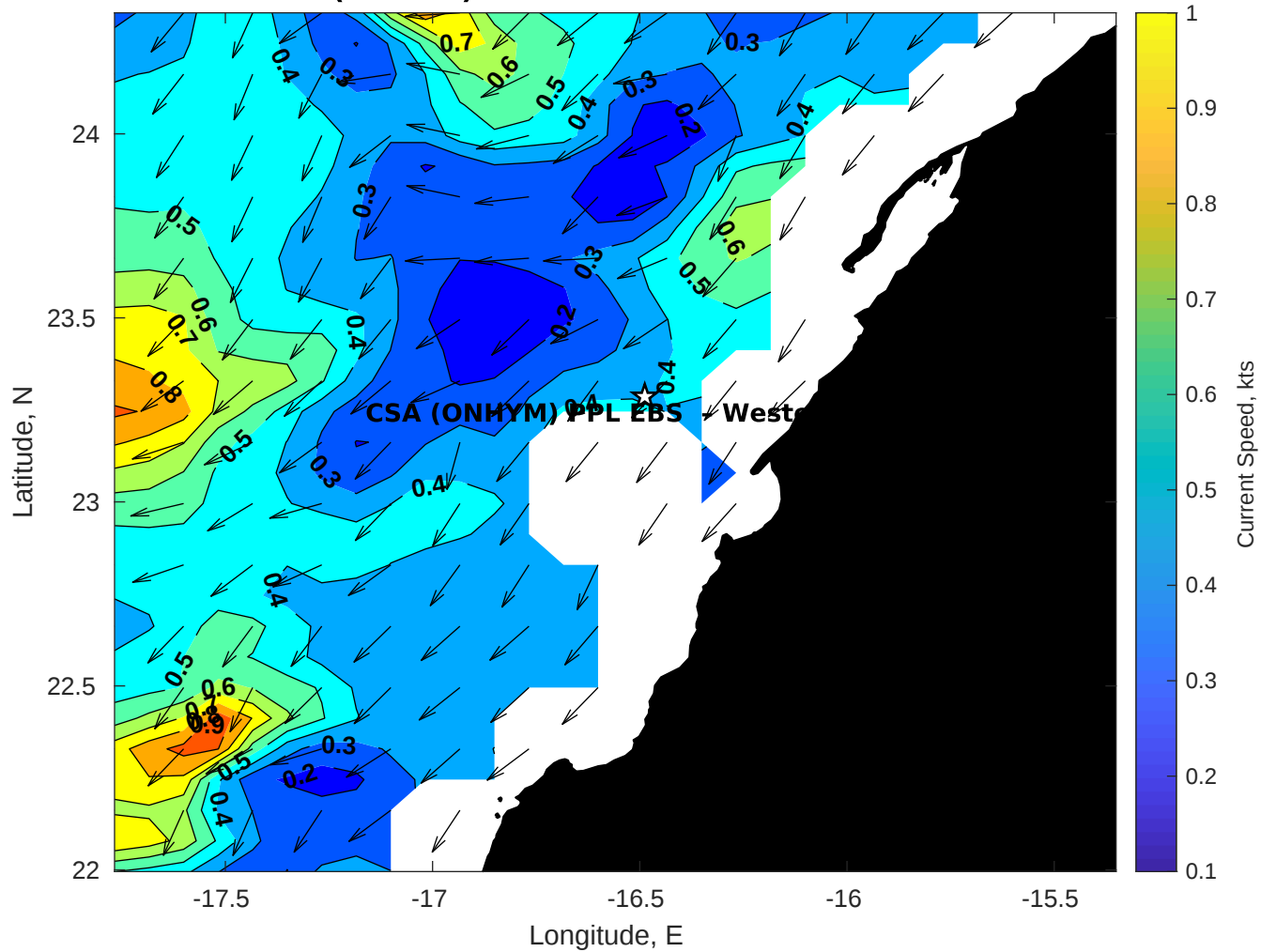
Surface Currents for CSA (ONHYM) PPL EBS - Western Sahara at 20-Dec-2025 00:00:00
