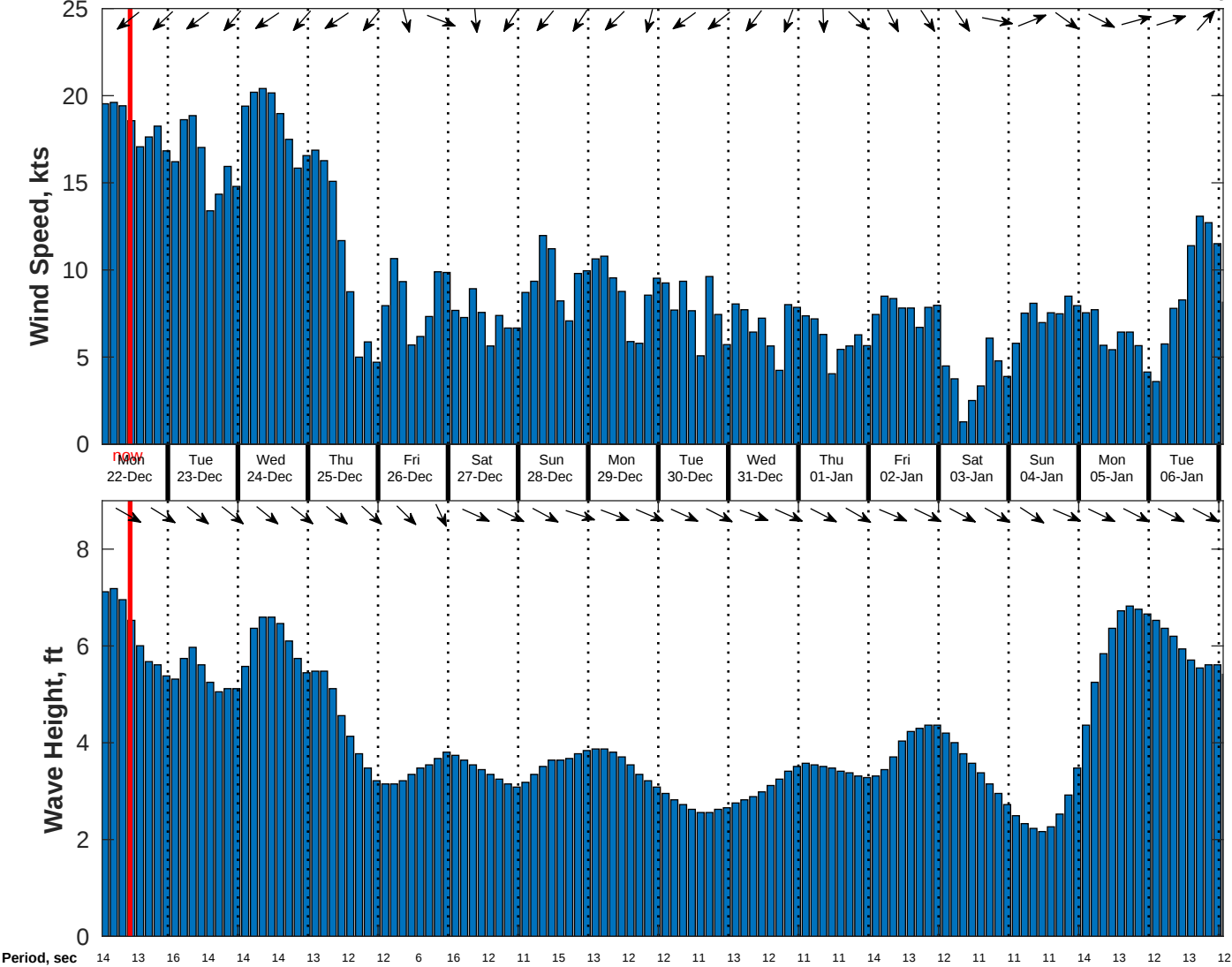
Wind & Wave Forecast for CSA (ONHYM) PPL EBS - Western Sahara from 21-Dec-2025 01:00:00 to 06-Jan-2026 01:00:00
