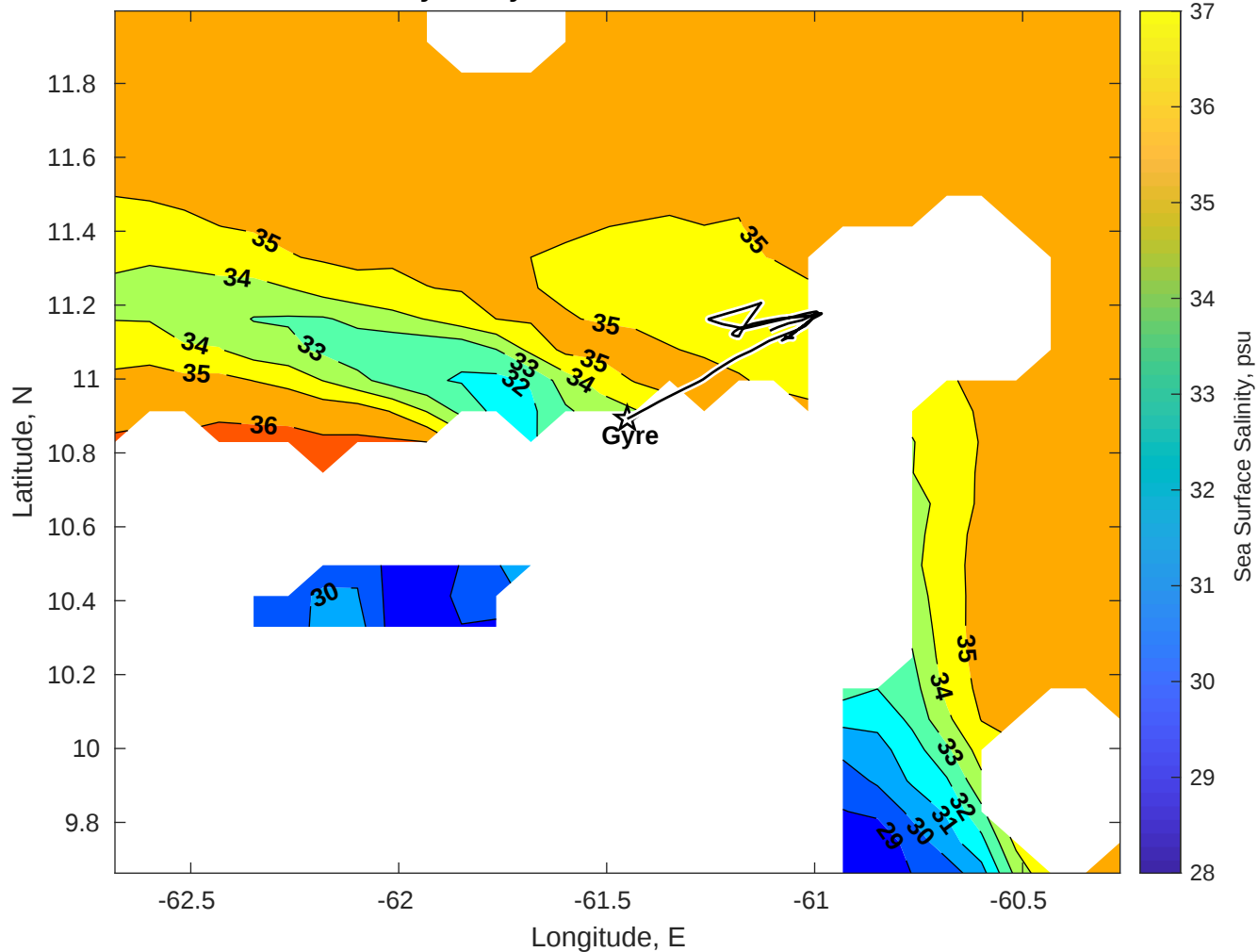
Surface Salinity for Gyre at 20-Dec-2025 00:00:00
