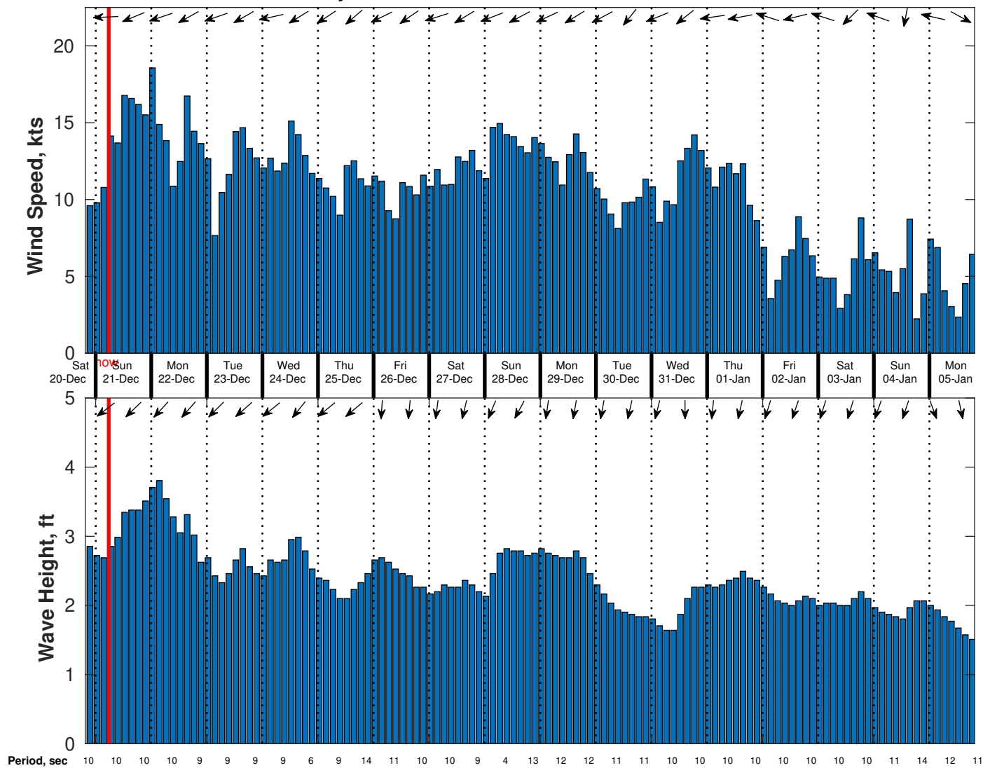
Wind & Wave Forecast for Gyre from 20-Dec-2025 20:00:00 to 05-Jan-2026 20:00:00
