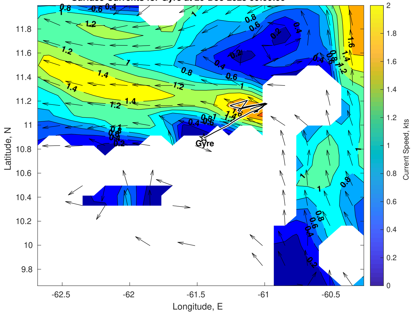
Surface Currents for Gyre at 20-Dec-2025 00:00:00
