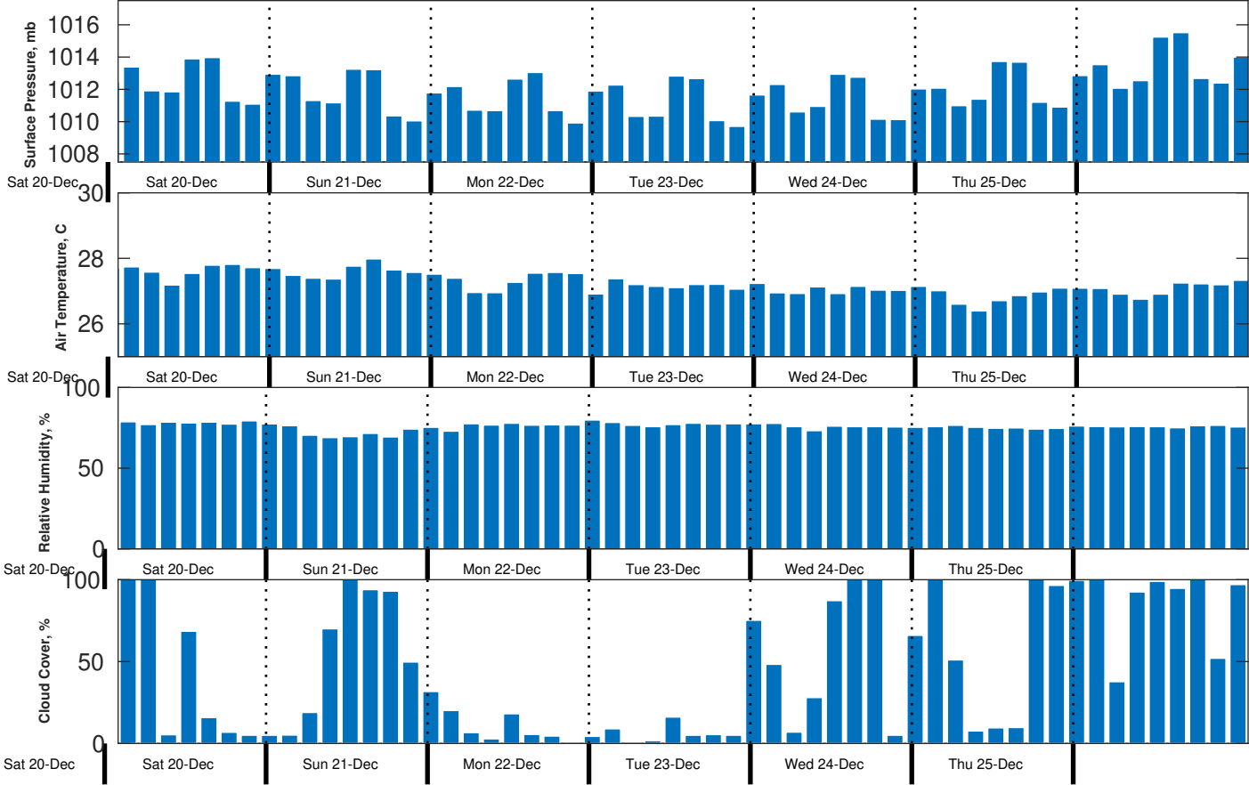
Met Forecast for Gyre from 20-Dec-2025 20:00:00 to 27-Dec-2025 20:00:00
