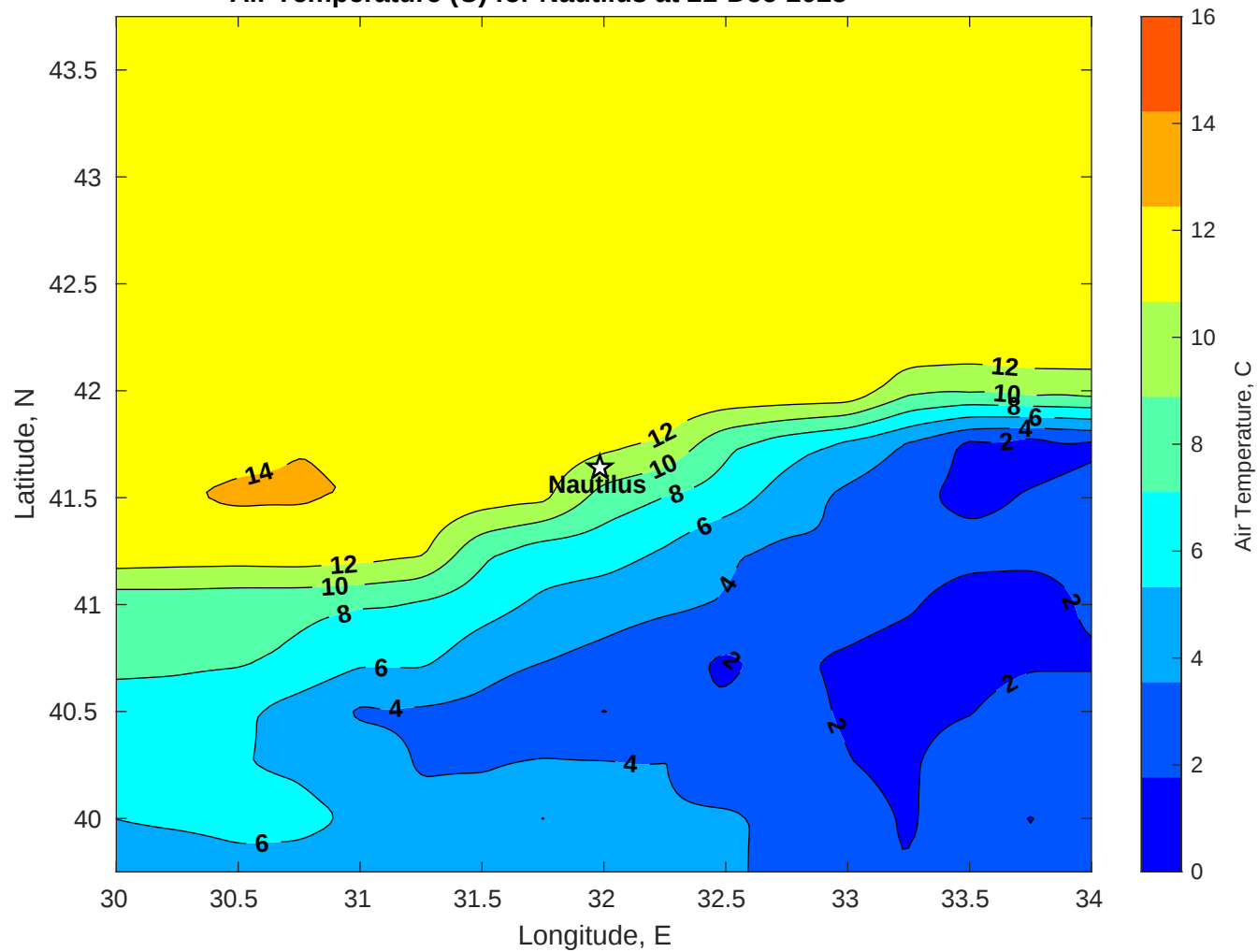
Air Temperature (C) for Nautilus at 21-Dec-2025
