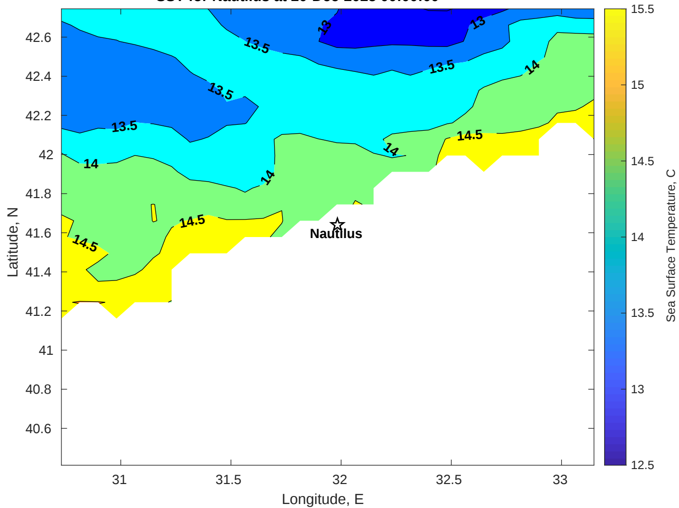
SST for Nautilus at 20-Dec-2025 00:00:00
